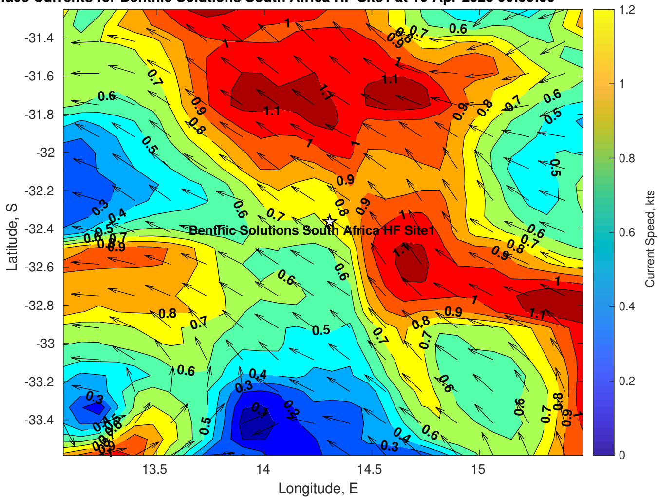
Surface Currents for Benthic Solutions South Africa HF Site1 at 16-Apr-2025 00:00:00
