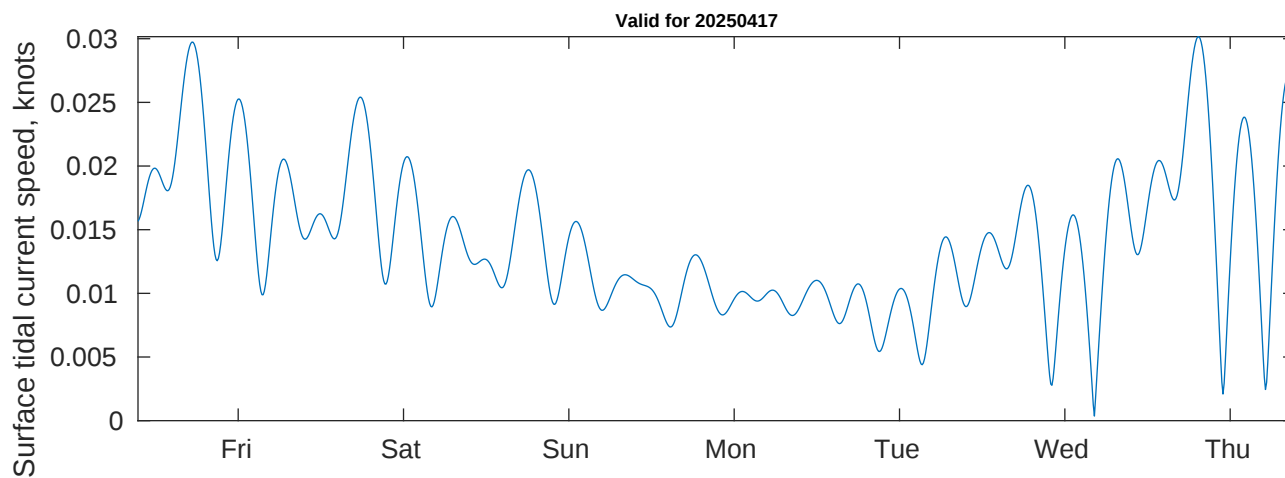
Tidal Currents and Heights for Benthic Solutions South Africa HF Site1 at 20250417
