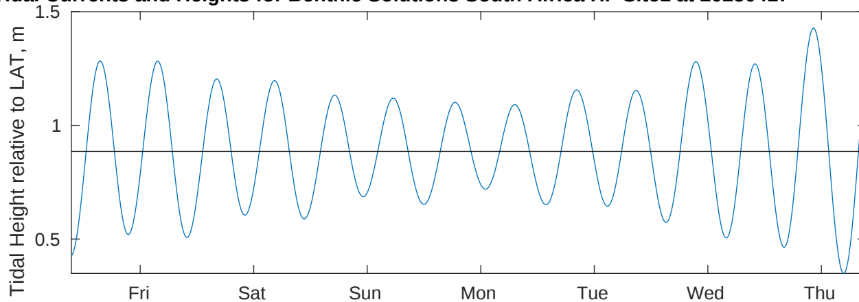
Tidal Currents and Heights for Benthic Solutions South Africa HF Site1 at 20250417
