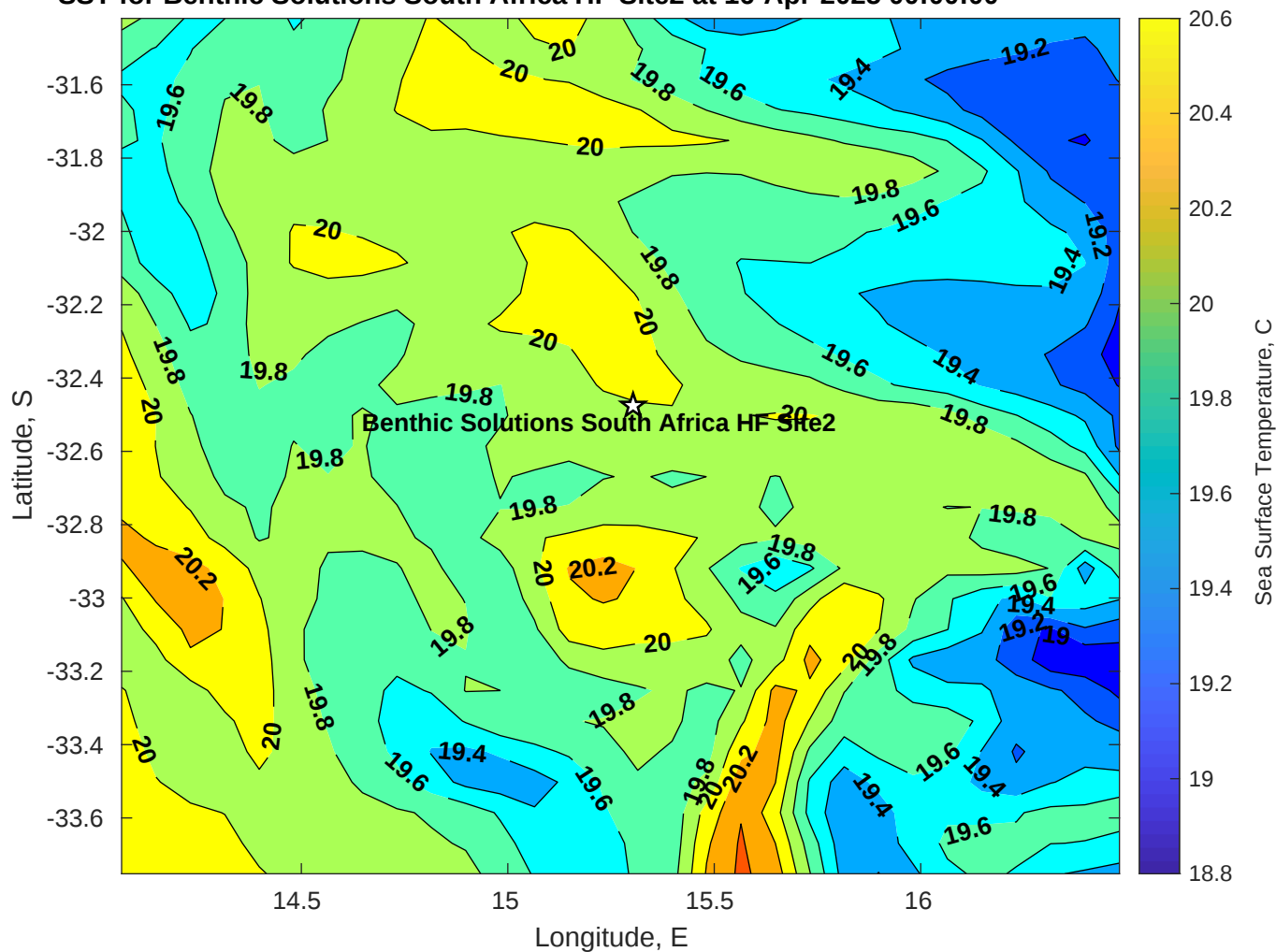
SST for Benthic Solutions South Africa HF Site2 at 16-Apr-2025 00:00:00
