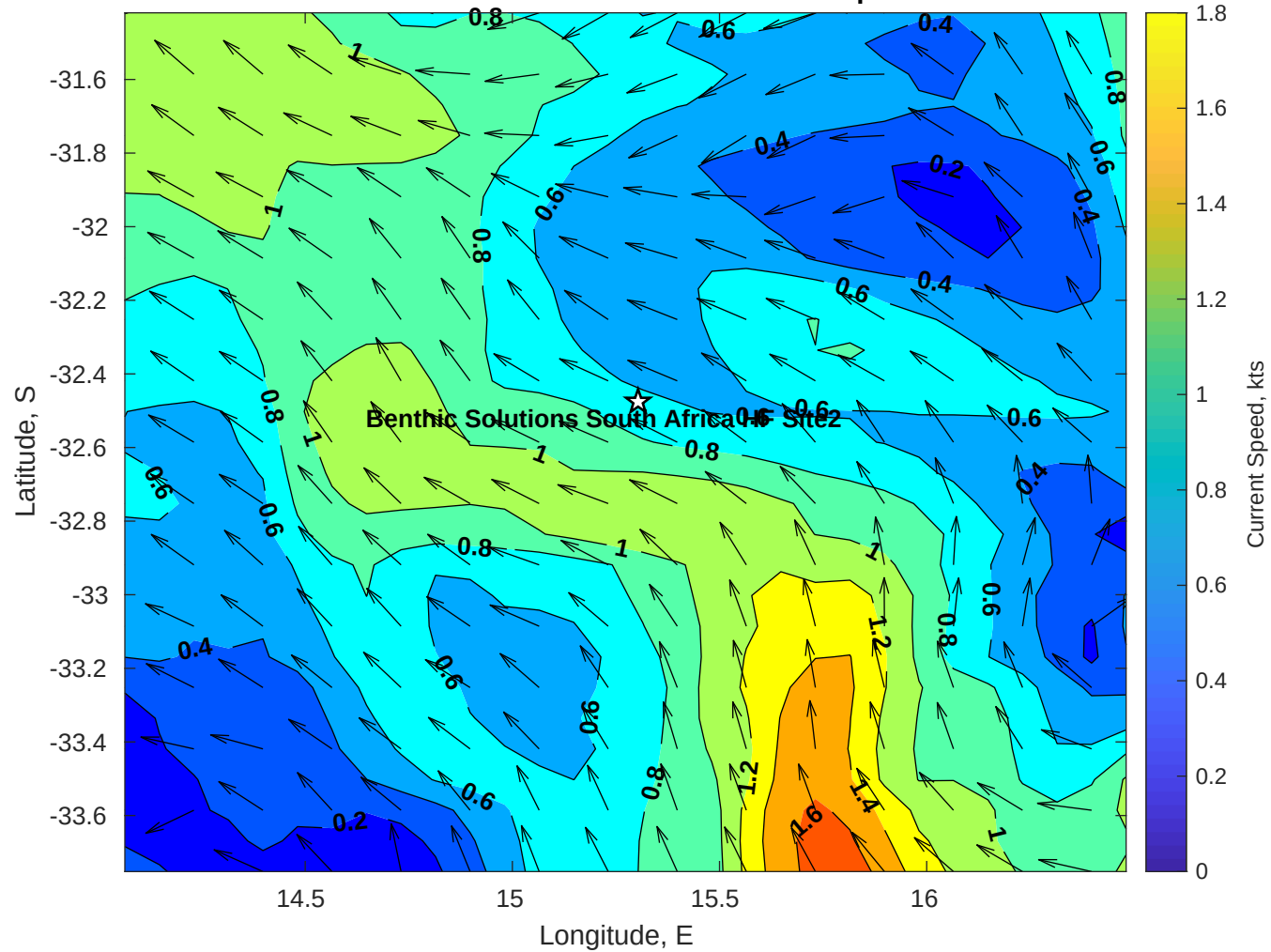
Surface Currents for Benthic Solutions South Africa HF Site2 at 16-Apr-2025 00:00:00
