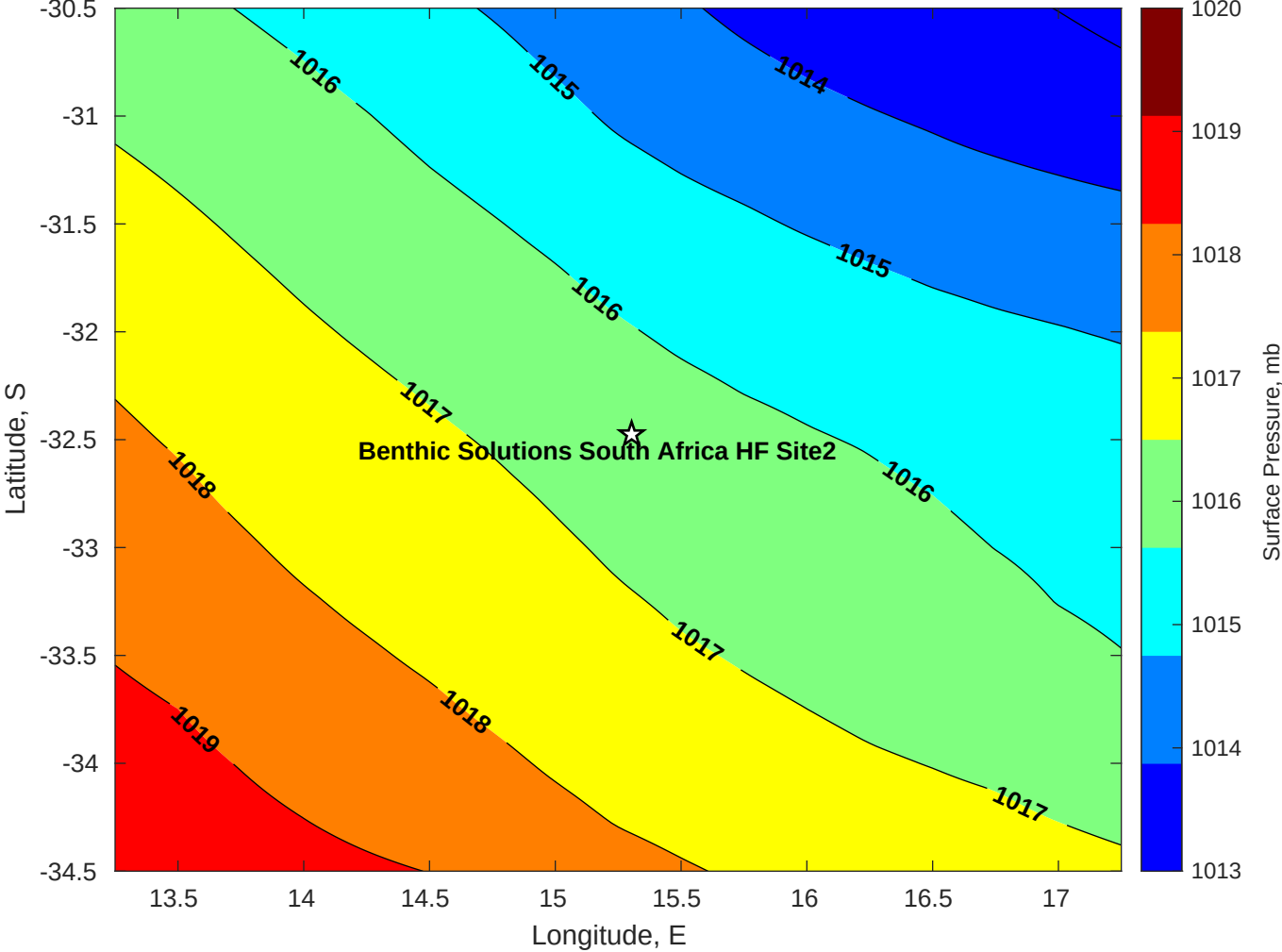
Surface Pressure (mb) for Benthic Solutions South Africa HF Site2 at 18-Apr-2025 00:00:00
