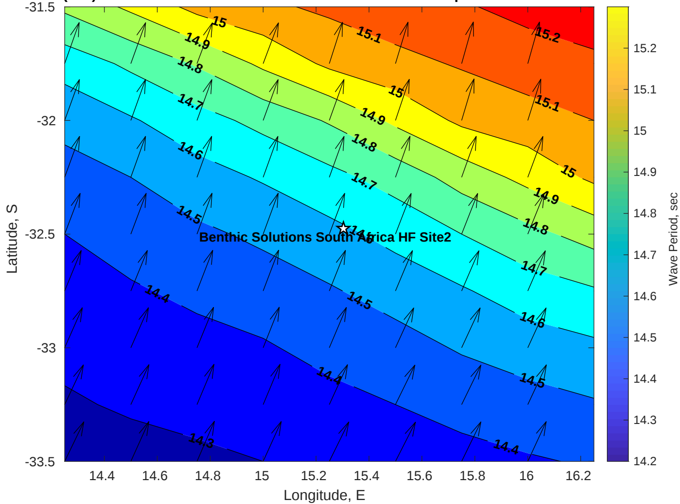
Wave Period (sec) for Benthic Solutions South Africa HF Site2 at 17-Apr-2025 09:00:00
