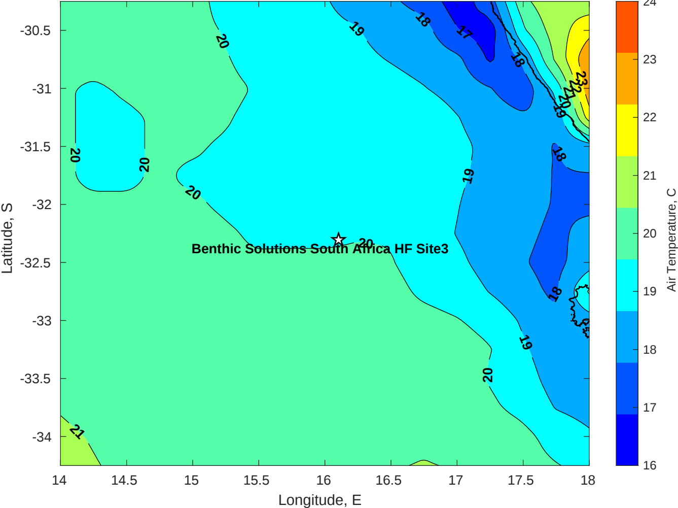
Air Temperature (C) for Benthic Solutions South Africa HF Site3 at 17-Apr-2025
