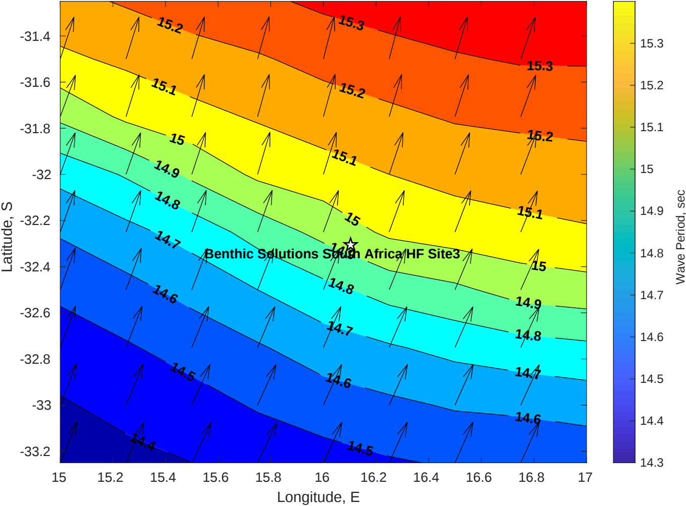
Wave Period (sec) for Benthic Solutions South Africa HF Site3 at 17-Apr-2025 09:00:00
