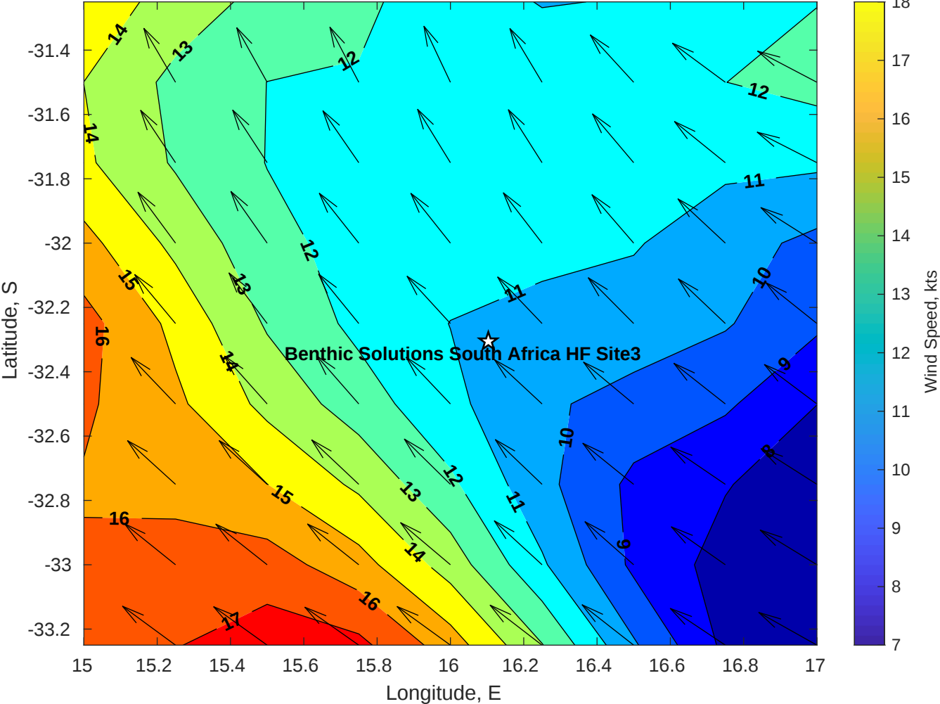
Winds (kts) for Benthic Solutions South Africa HF Site3 at 17-Apr-2025 09:00:00
