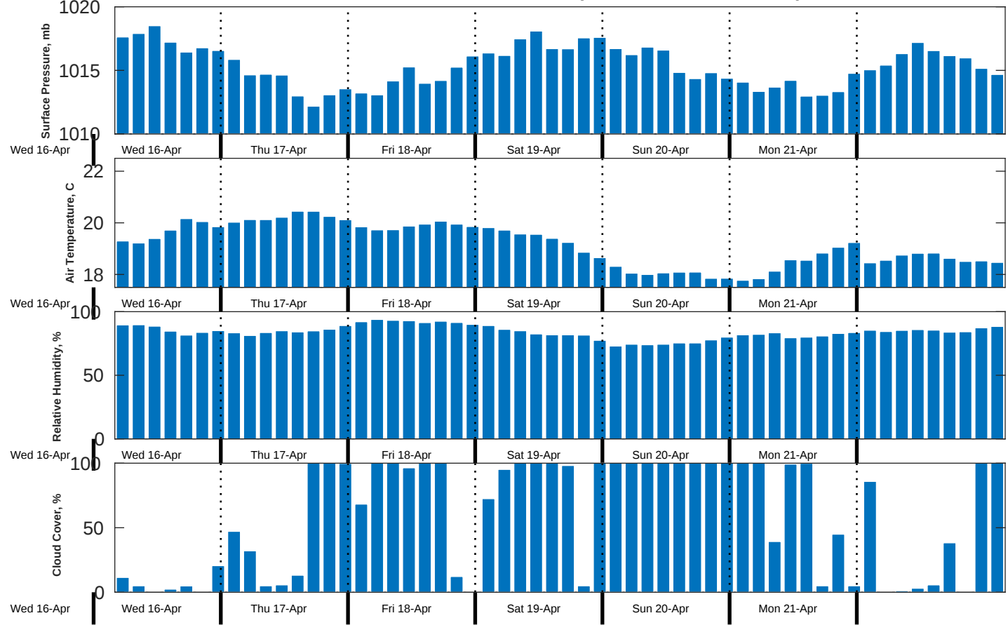
Met Forecast for Benthic Solutions South Africa HF Site3 from 17-Apr-2025 00:00:00 to 24-Apr-2025 00:00:00
