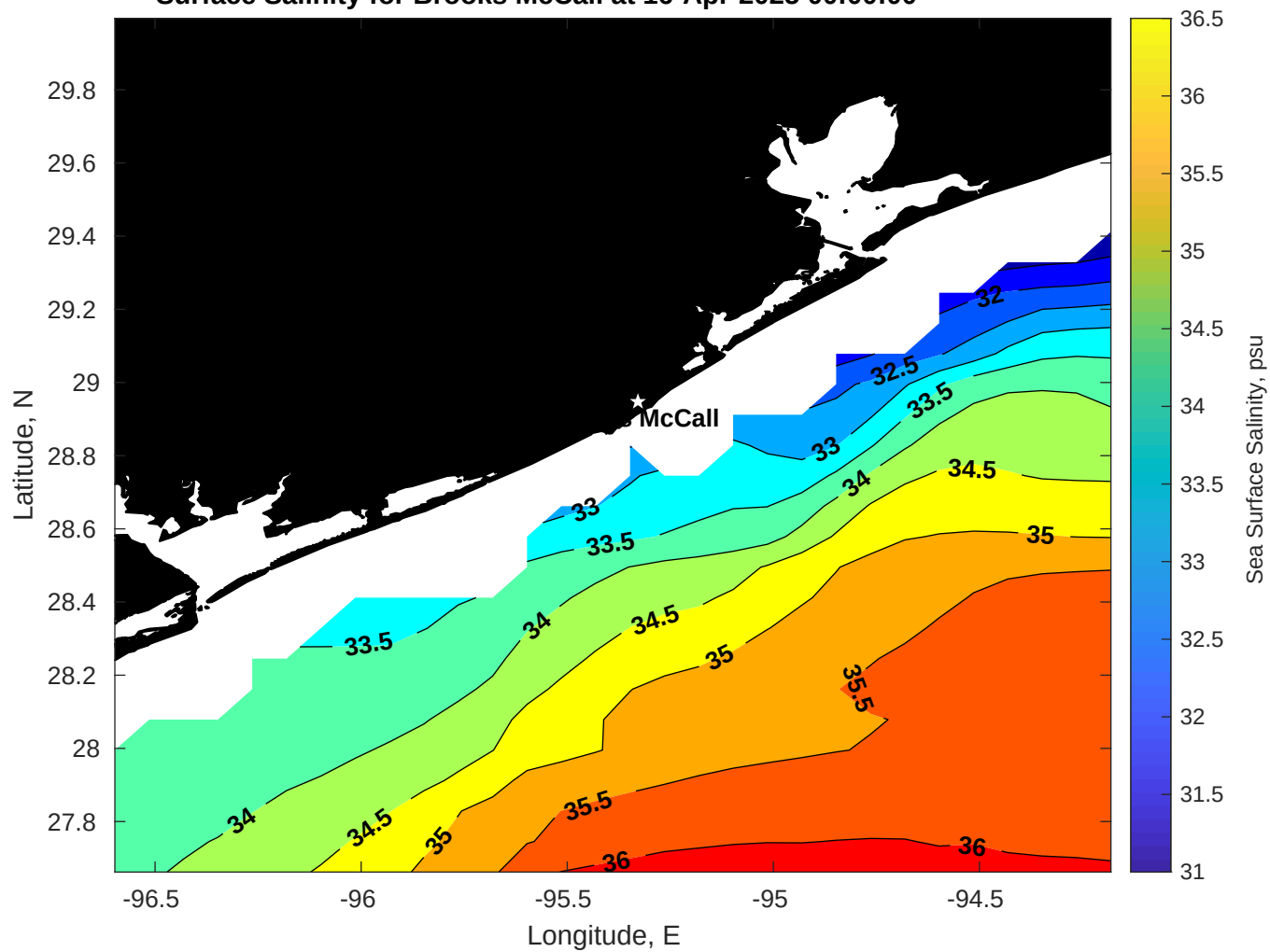
Surface Salinity for Brooks McCall at 16-Apr-2025 00:00:00
