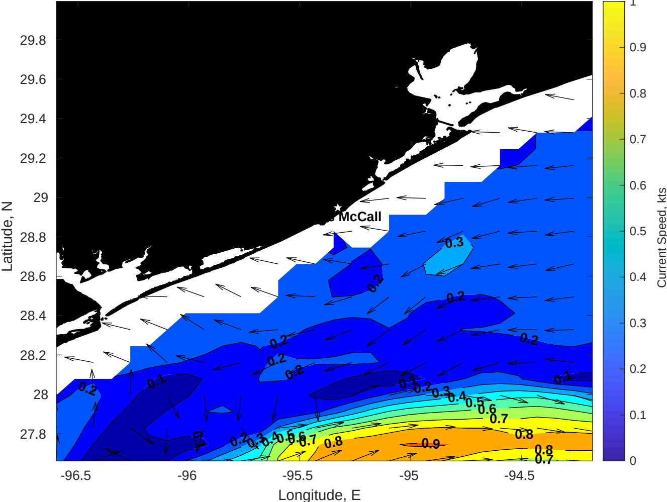
Surface Currents for Brooks McCall at 16-Apr-2025 00:00:00
