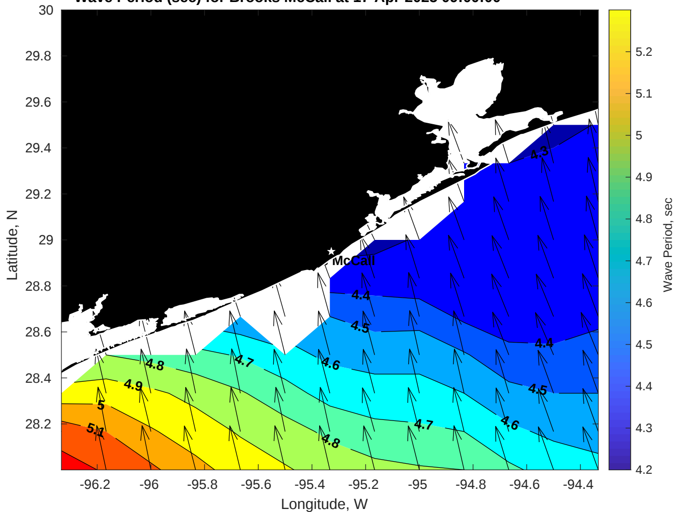
Wave Period (sec) for Brooks McCall at 17-Apr-2025 09:00:00
