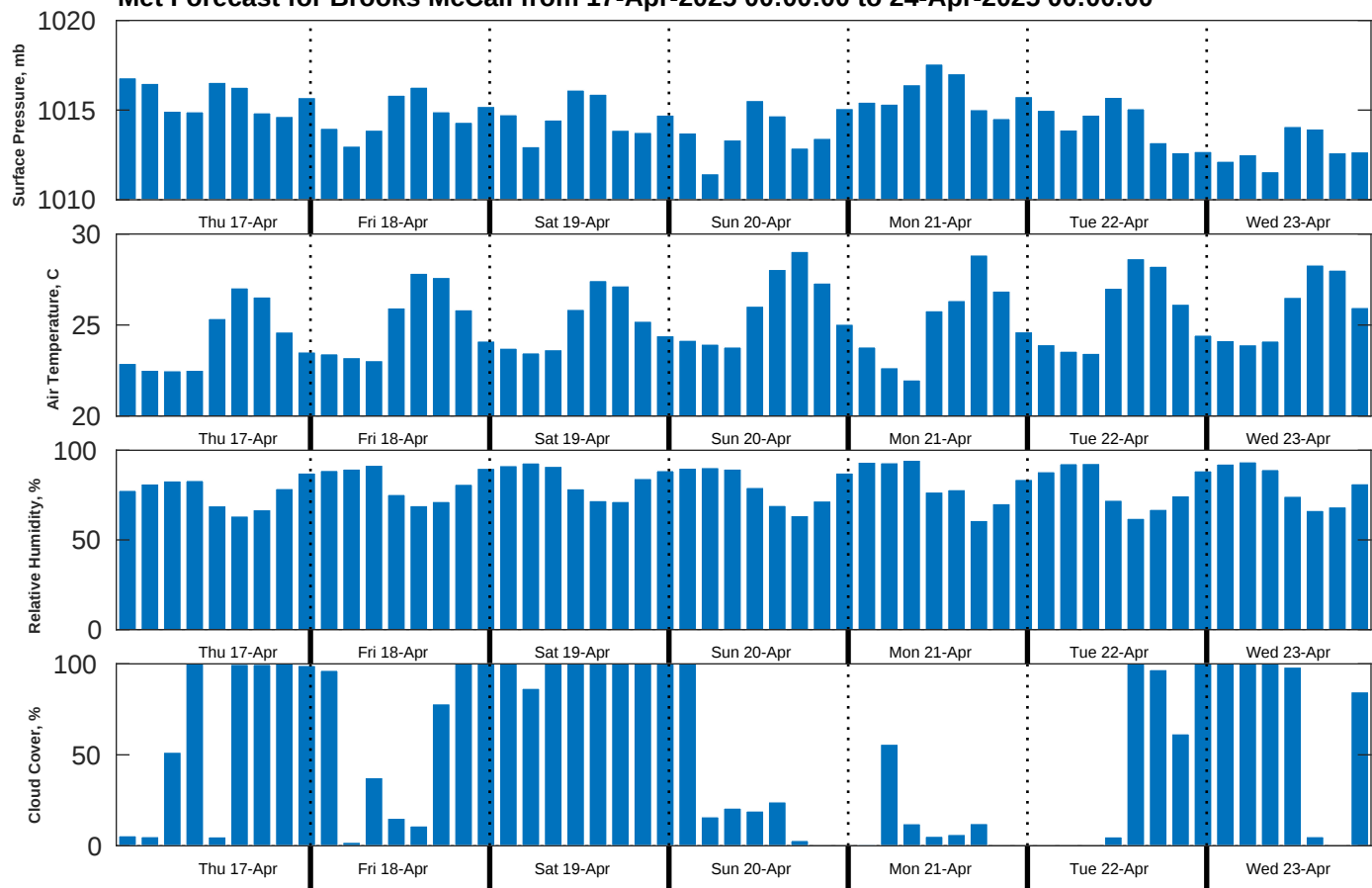
Met Forecast for Brooks McCall from 17-Apr-2025 00:00:00 to 24-Apr-2025 00:00:00
