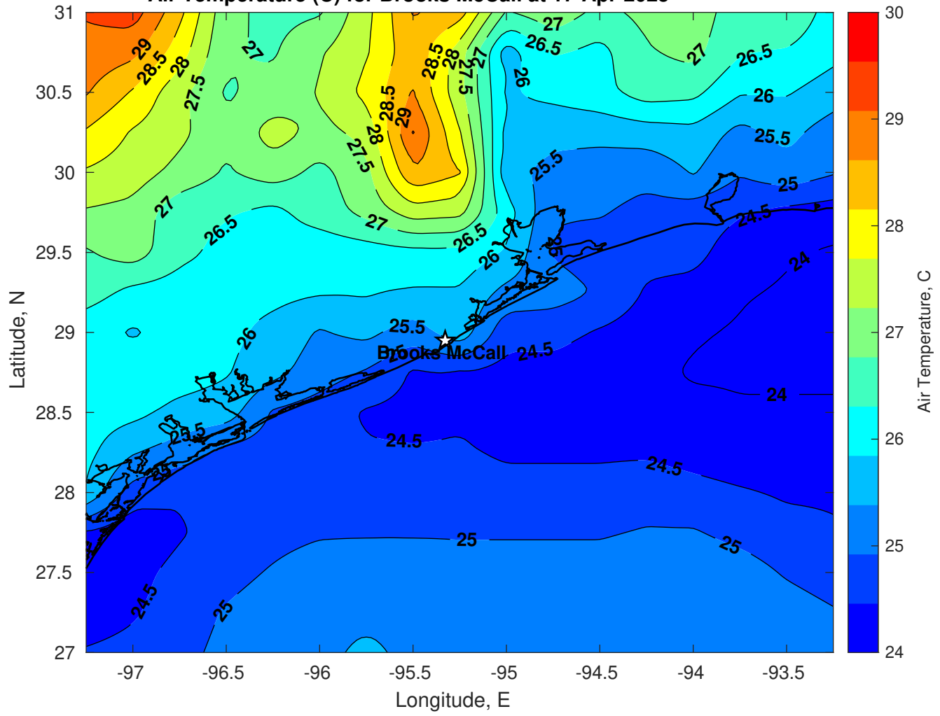
Air Temperature (C) for Brooks McCall at 17-Apr-2025
