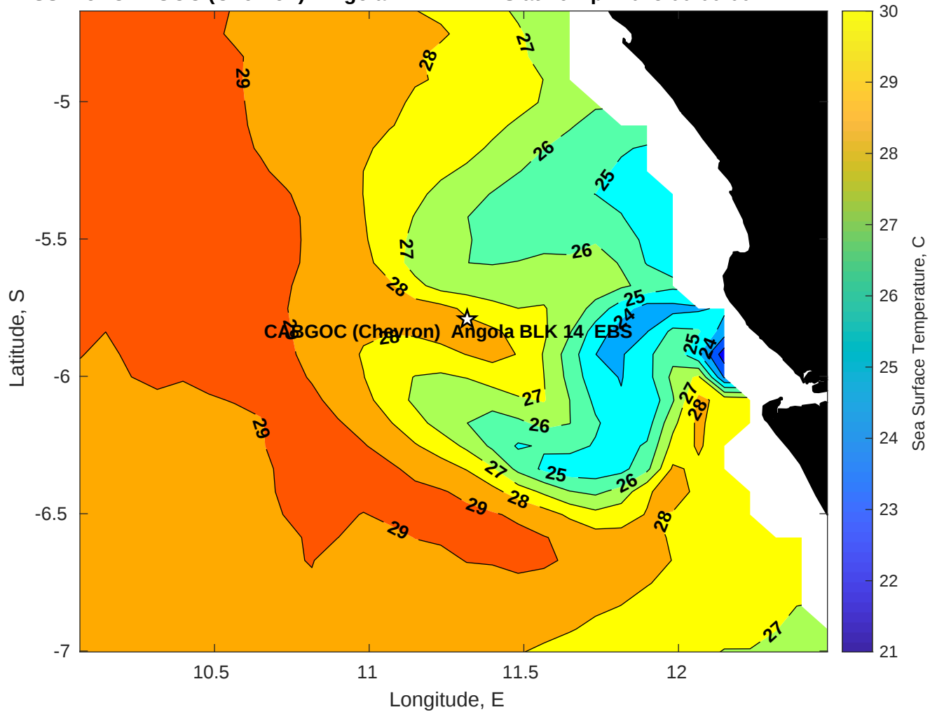
SST for CABGOC (Chevron) Angola BLK 14 EBS at 16-Apr-2025 00:00:00
