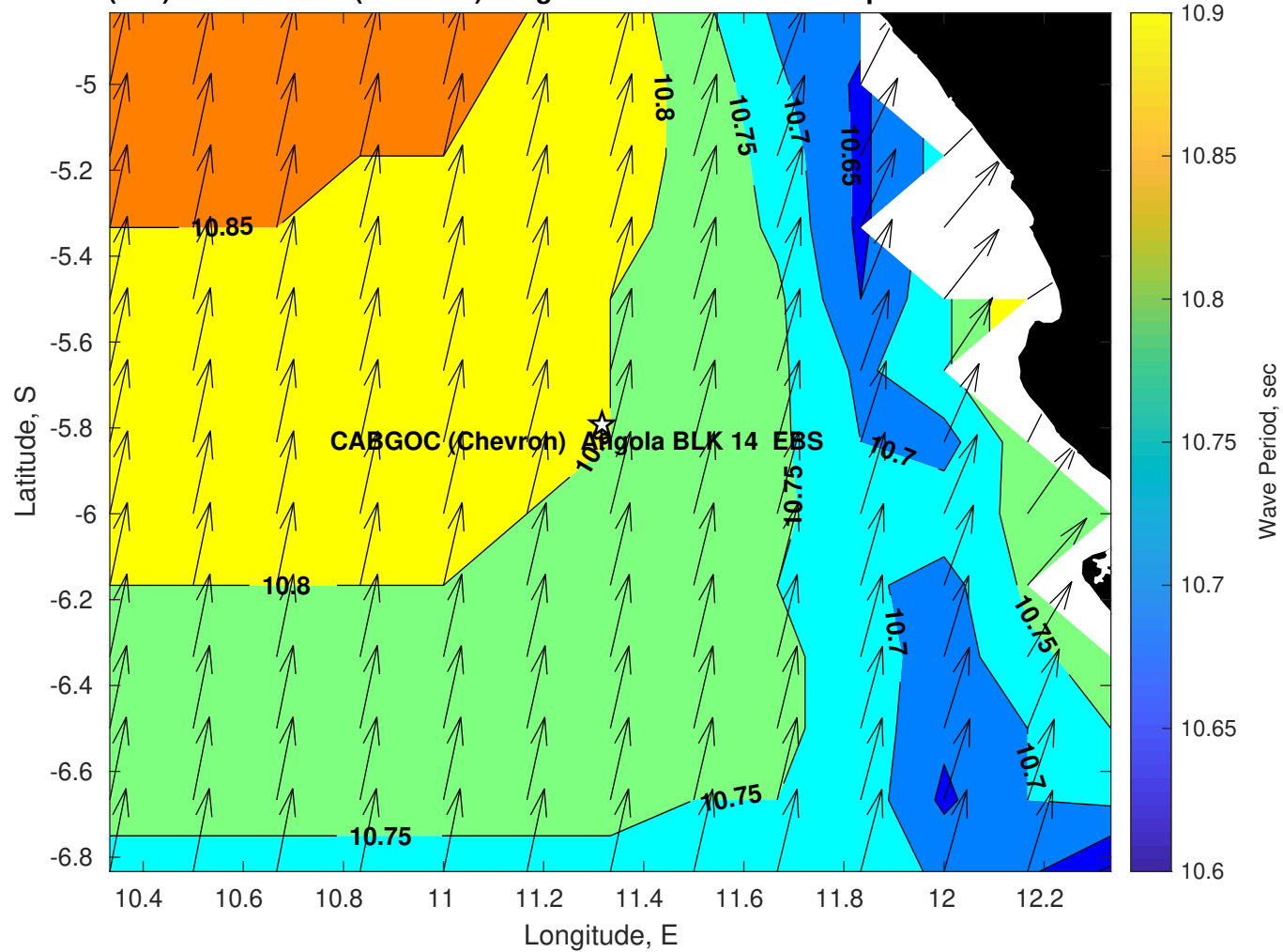
Wave Period (sec) for CABGOC (Chevron) Angola BLK 14 EBS at 17-Apr-2025 09:00:00
