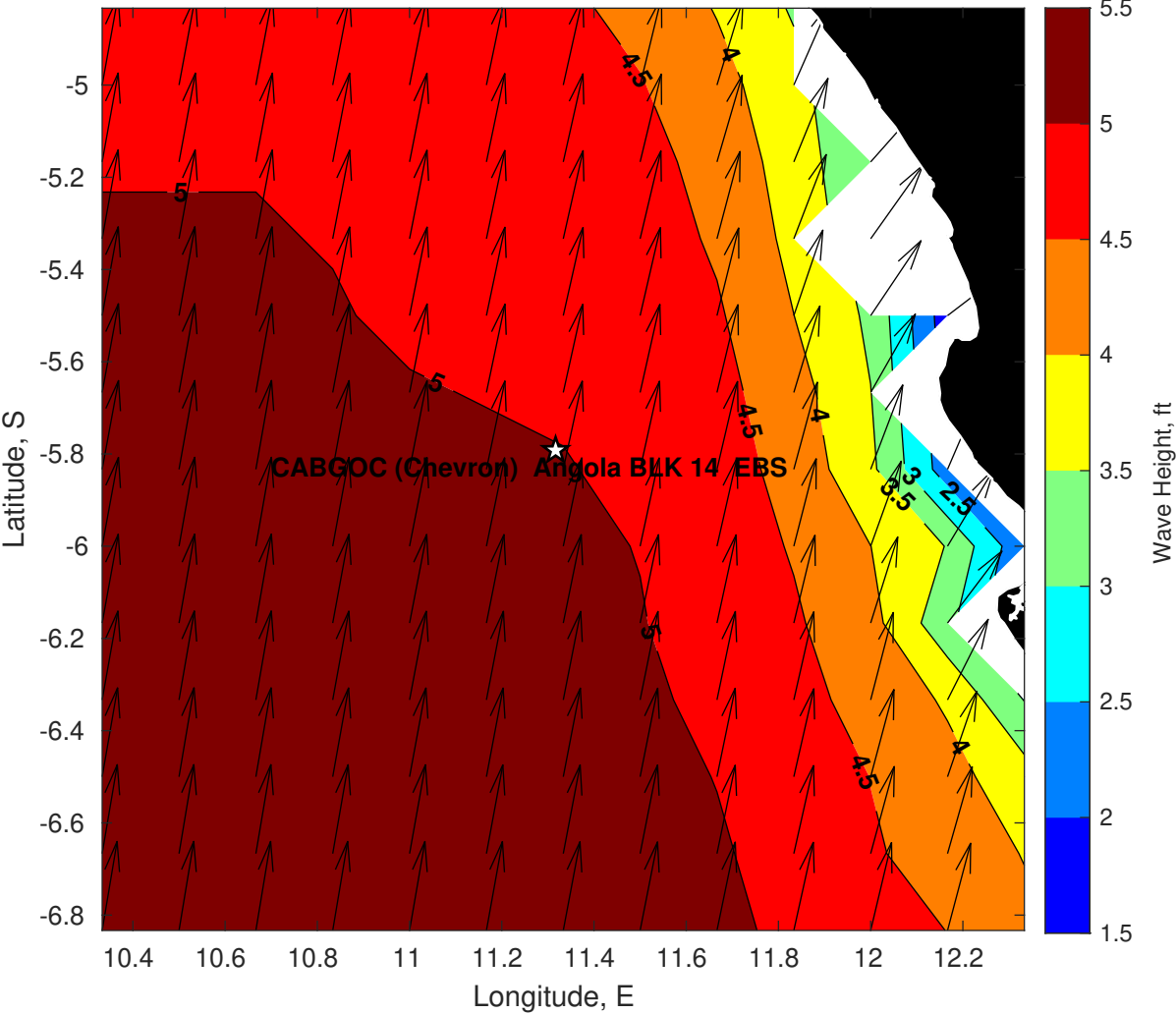
Wave Height (ft) for CABGOC (Chevron) Angola BLK 14 EBS at 17-Apr-2025 09:00:00
