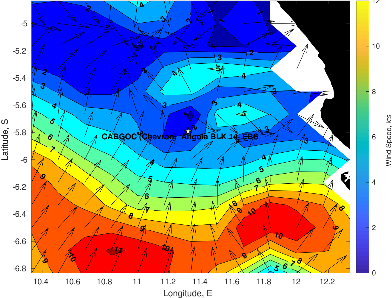
Winds (kts) for CABGOC (Chevron) Angola BLK 14 EBS at 17-Apr-2025 09:00:00
