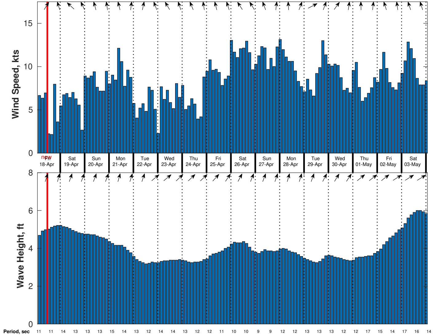
Wind & Wave Forecast for CABGOC (Chevron) Angola BLK 14 EBS from 17-Apr-2025 02:00:00 to 03-May-2025 02:00:00
