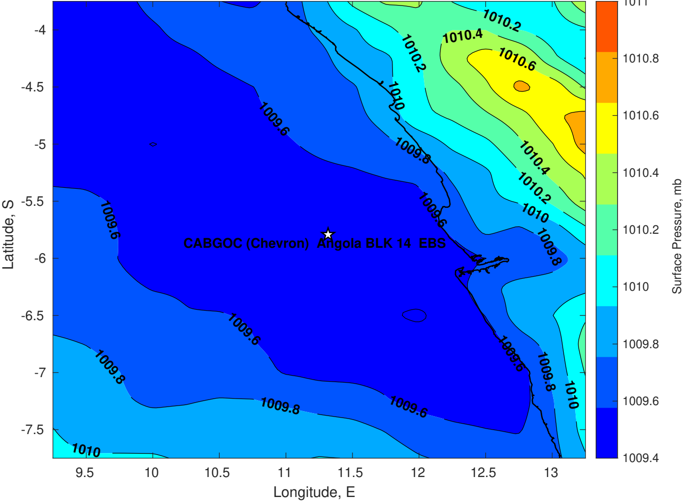
Surface Pressure (mb) for CABGOC (Chevron) Angola BLK 14 EBS at 19-Apr-2025 00:00:00
