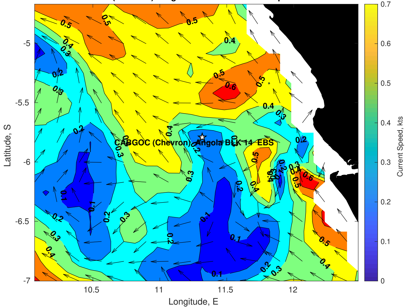
Surface Currents for CABGOC (Chevron) Angola BLK 14 EBS at 16-Apr-2025 00:00:00
