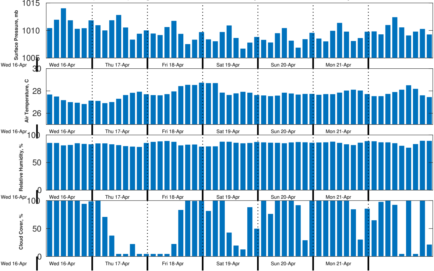
Met Forecast for CABGOC (Chevron) Angola BLK 14 EBS from 17-Apr-2025 00:00:00 to 24-Apr-2025 00:00:00
