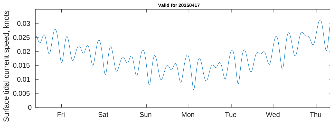
Tidal Currents and Heights for CABGOC (Chevron) Angola BLK 14 EBS at 20250417
