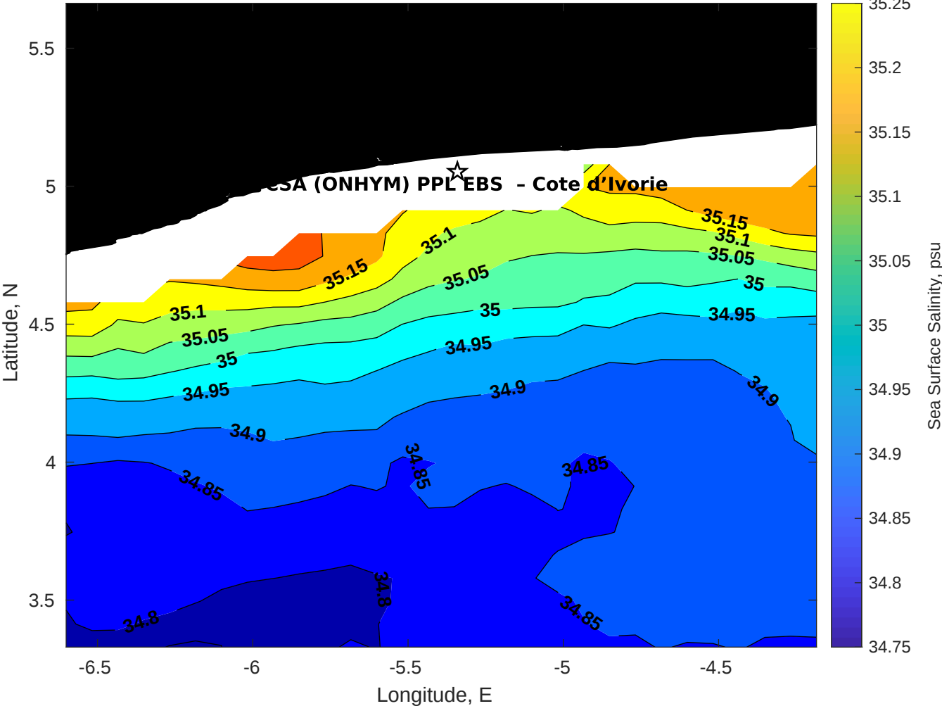
Surface Salinity for CSA (ONHYM) PPL EBS - Cote d'Ivoire at 16-Apr-2025 00:00:00
