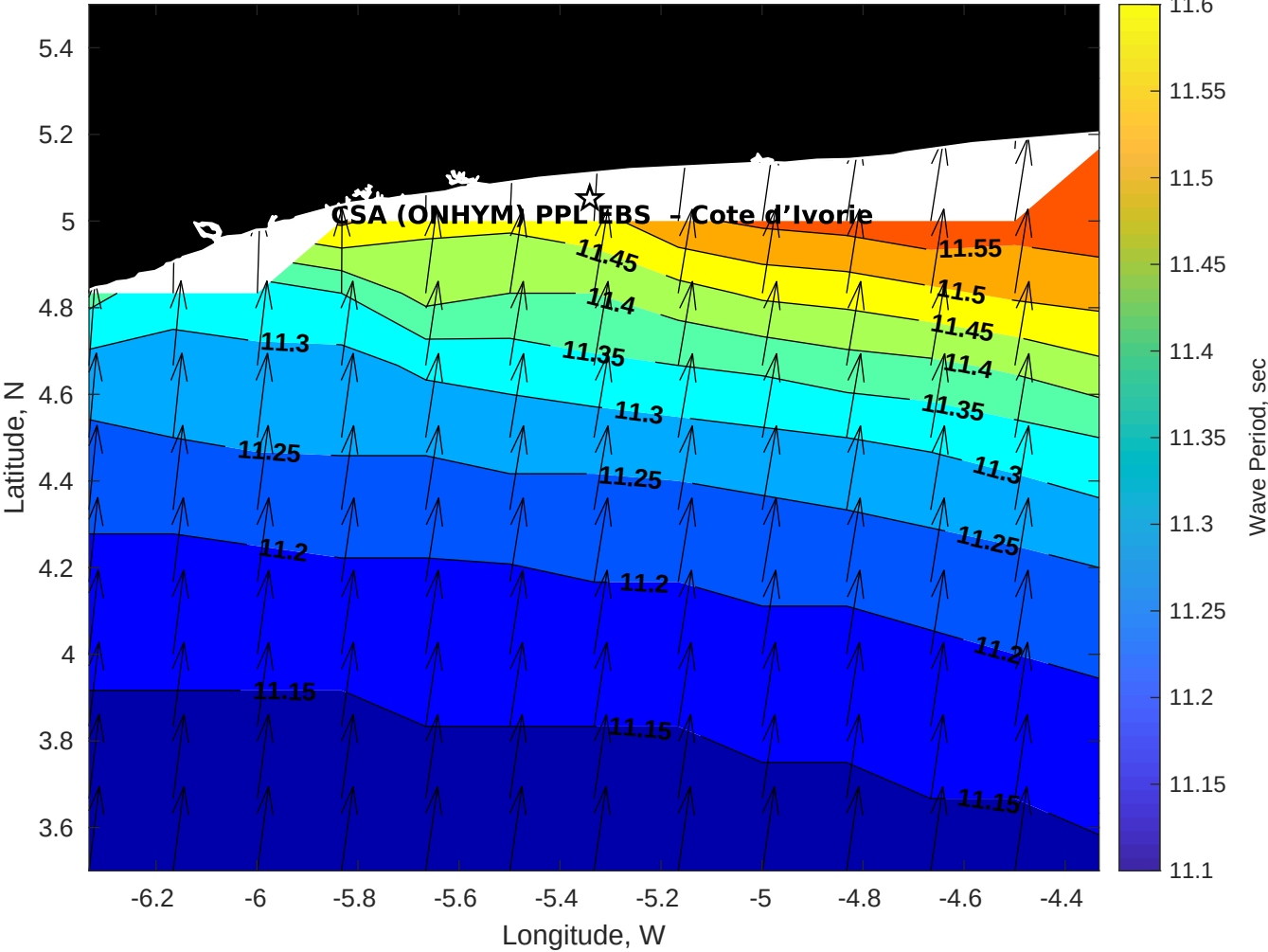
Wave Period (sec) for CSA (ONHYM) PPL EBS - Cote d'Ivoire at 17-Apr-2025 09:00:00
