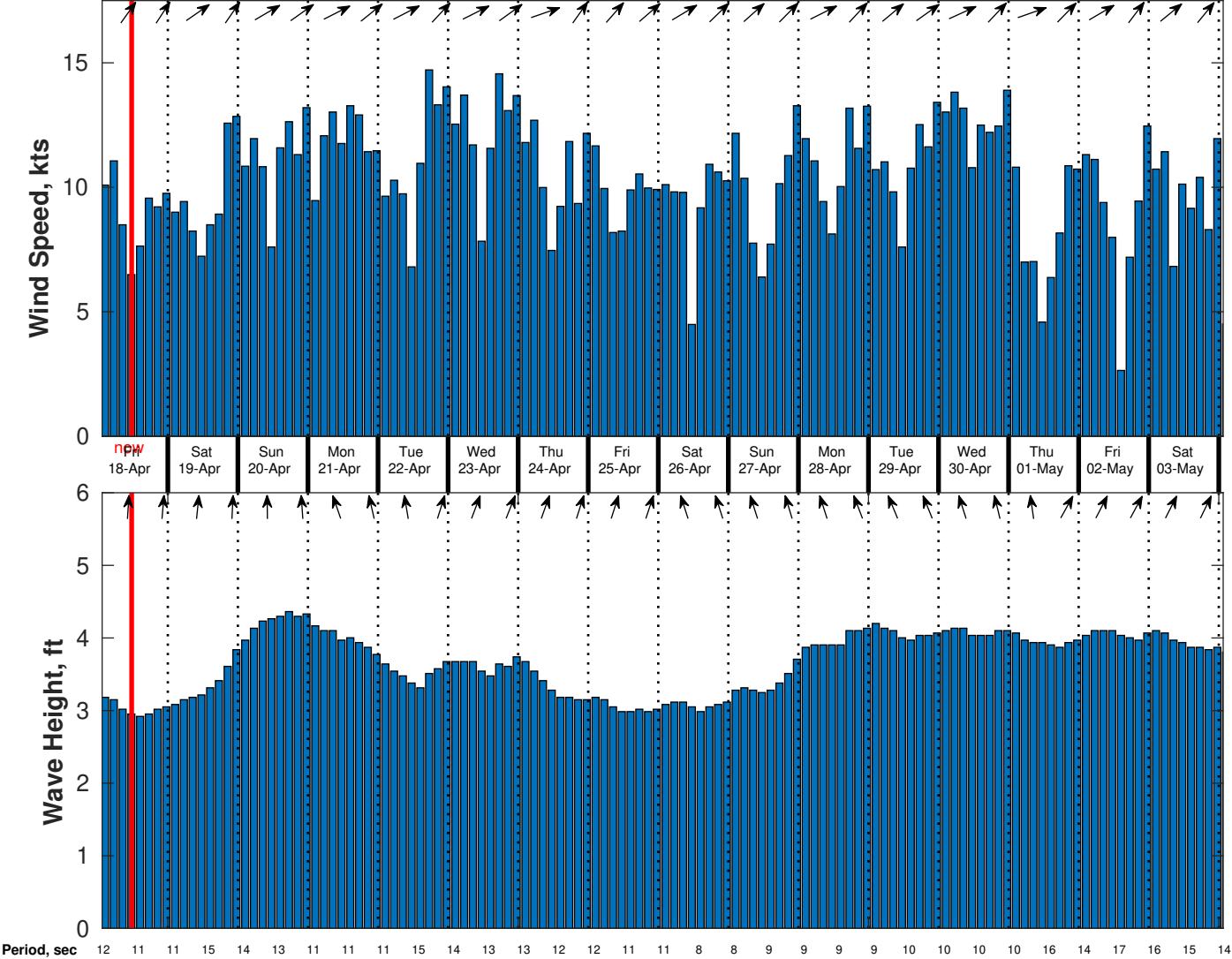
Wind & Wave Forecast for CSA (ONHYM) PPL EBS - Cote d'Ivoire from 17-Apr-2025 01:00:00 to 03-May-2025 01:00:00
