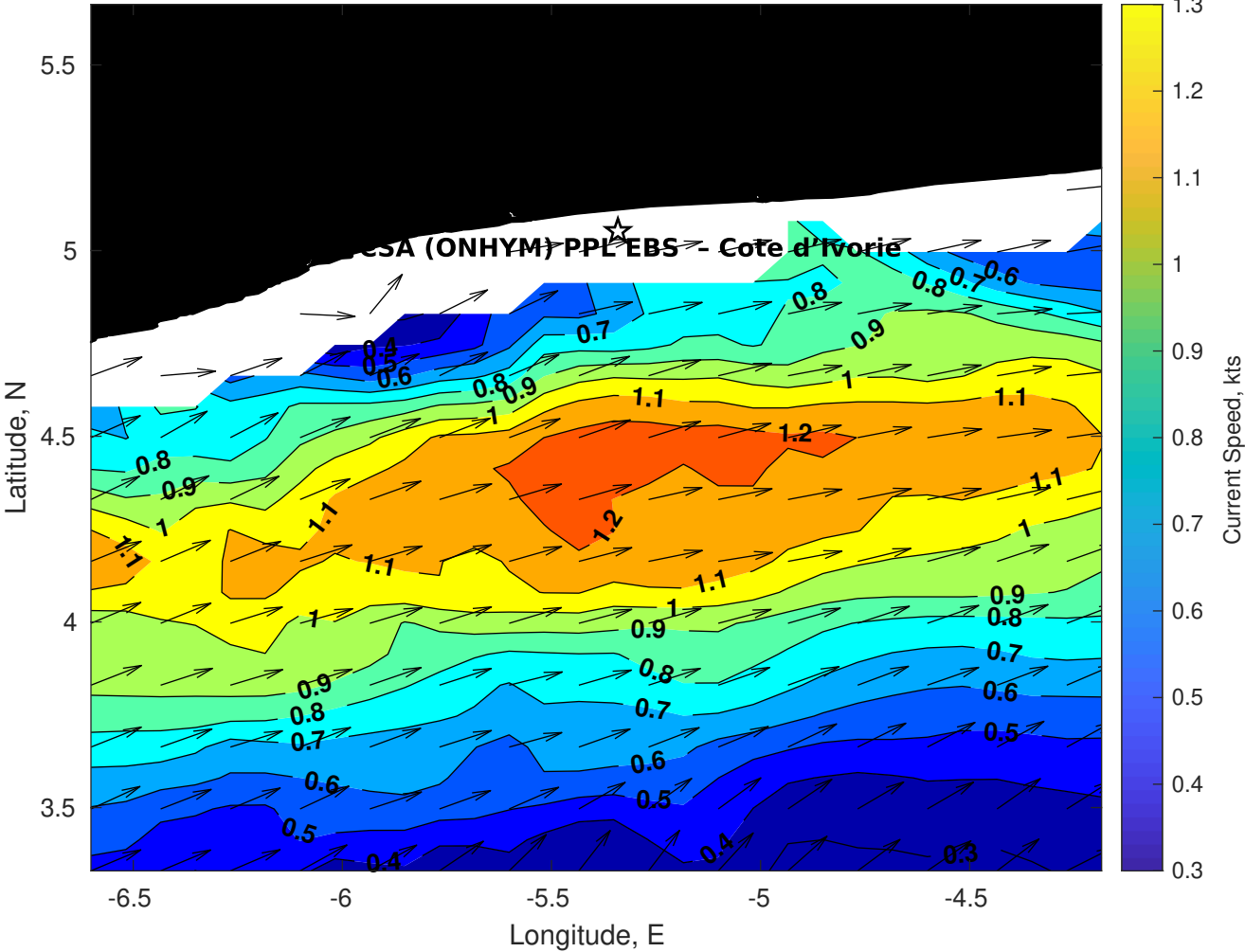
Surface Currents for CSA (ONHYM) PPL EBS - Cote d'Ivoire at 16-Apr-2025 00:00:00
