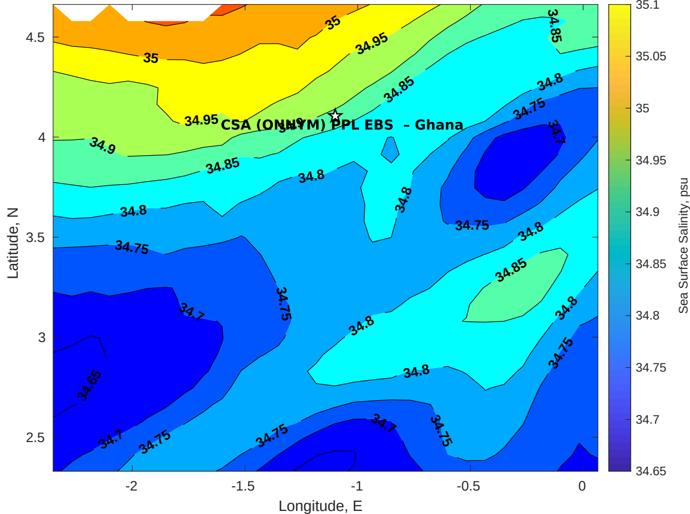
Surface Salinity for CSA (ONHYM) PPL EBS - Ghana at 16-Apr-2025 00:00:00
