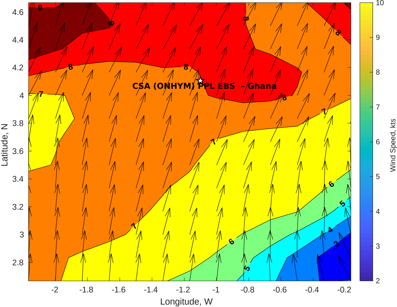
Winds (kts) for CSA (ONHYM) PPL EBS - Ghana at 17-Apr-2025 09:00:00
