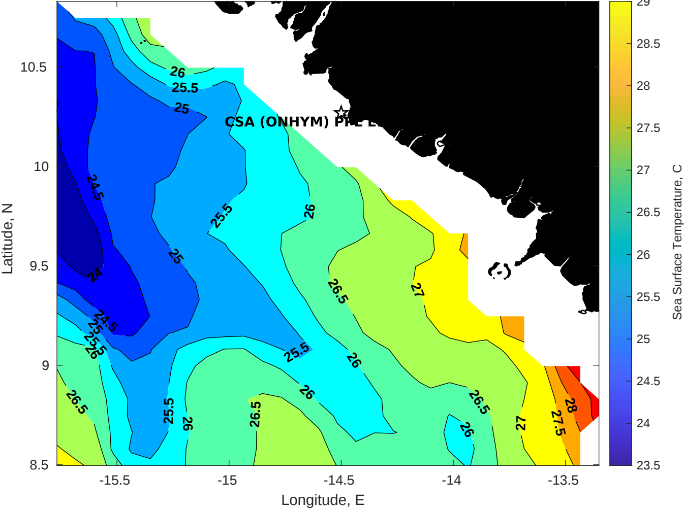
SST for CSA (ONHYM) PPL EBS - Guinea at 16-Apr-2025 00:00:00
