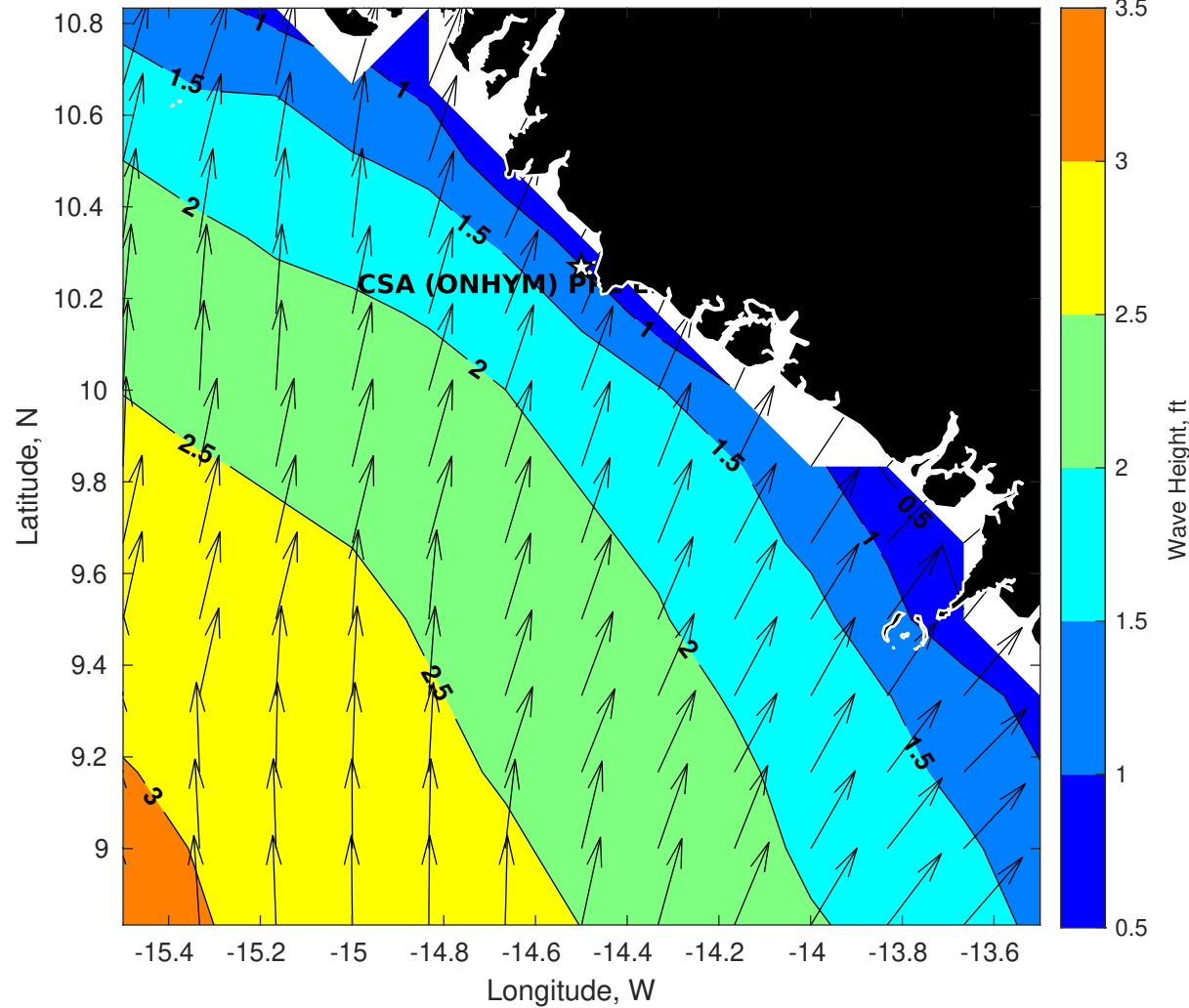
Wave Height (ft) for CSA (ONHYM) PPL EBS - Guinea at 17-Apr-2025 09:00:00
