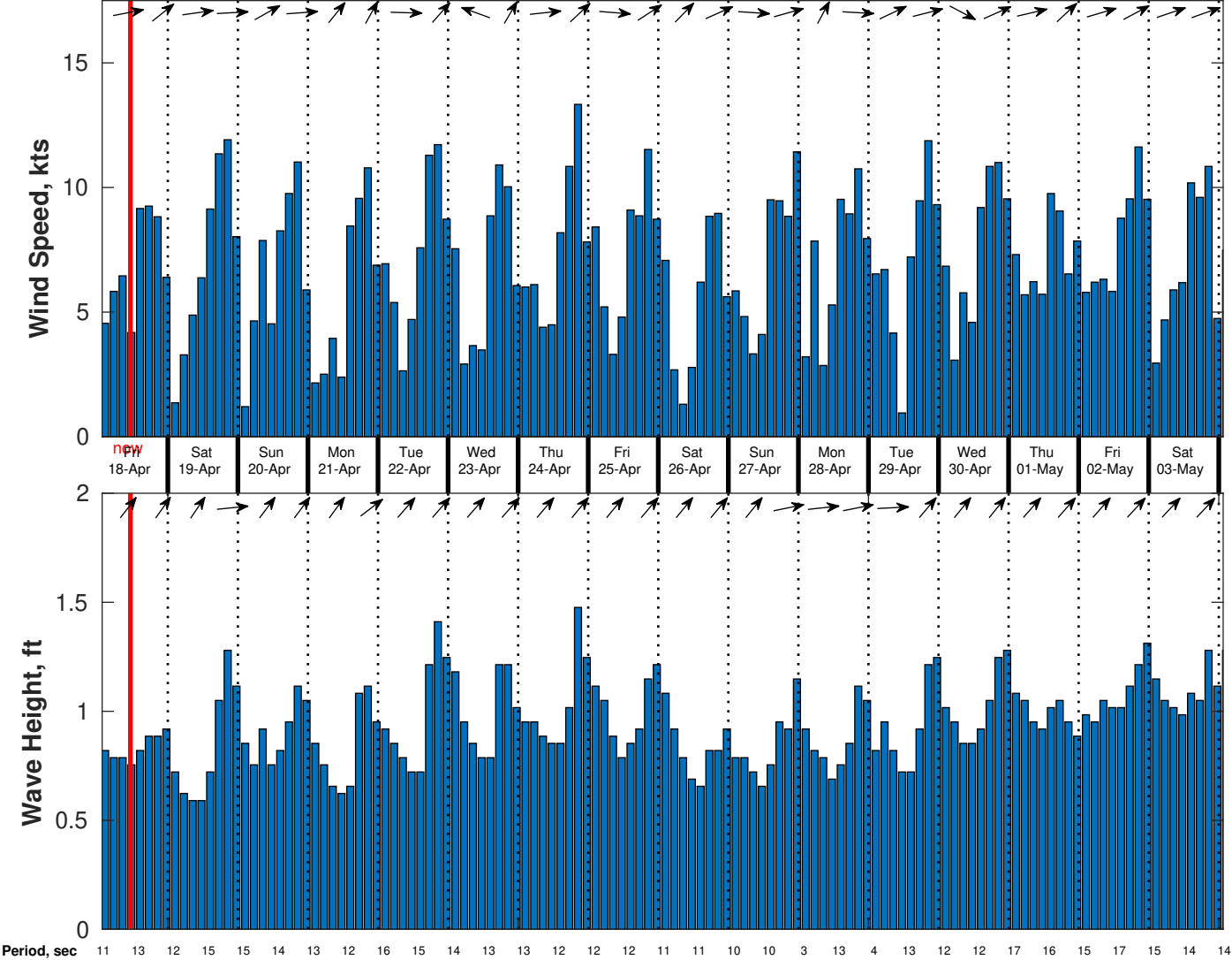
Wind & Wave Forecast for CSA (ONHYM) PPL EBS - Guinea from 17-Apr-2025 01:00:00 to 03-May-2025 01:00:00
