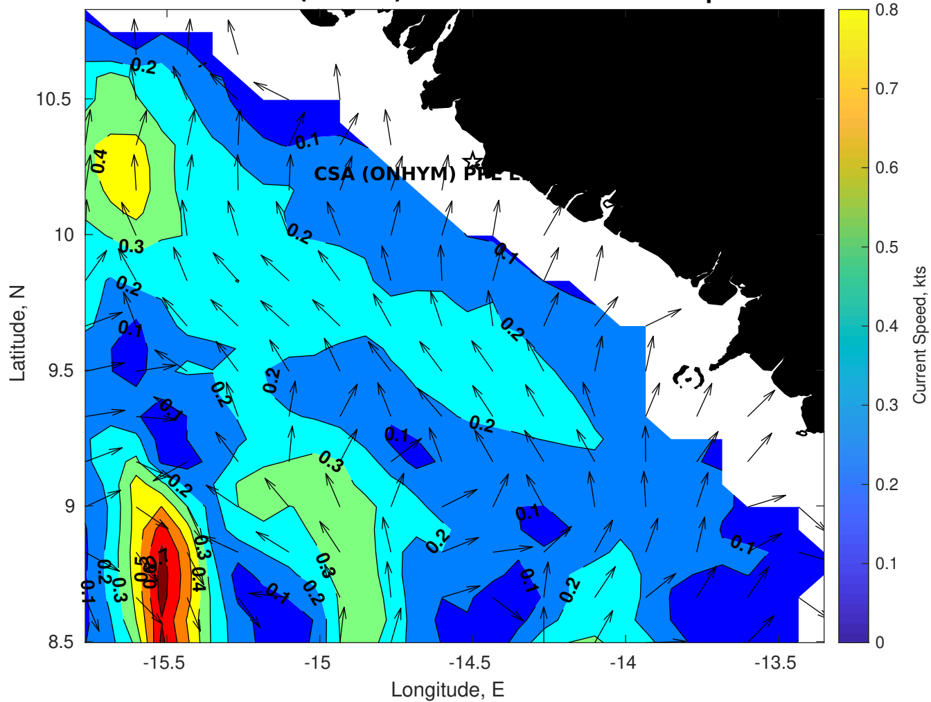
Surface Currents for CSA (ONHYM) PPL EBS - Guinea at 16-Apr-2025 00:00:00
