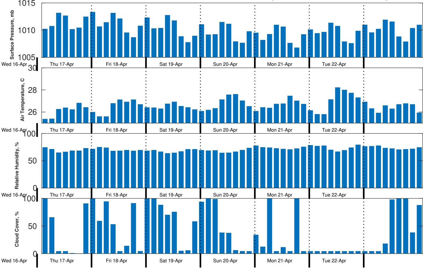
Met Forecast for CSA (ONHYM) PPL EBS - Guinea from 17-Apr-2025 00:00:00 to 24-Apr-2025 00:00:00
