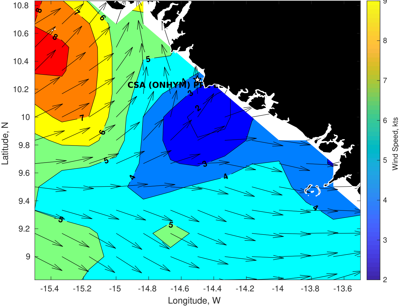
Winds (kts) for CSA (ONHYM) PPL EBS - Guinea at 17-Apr-2025 09:00:00
