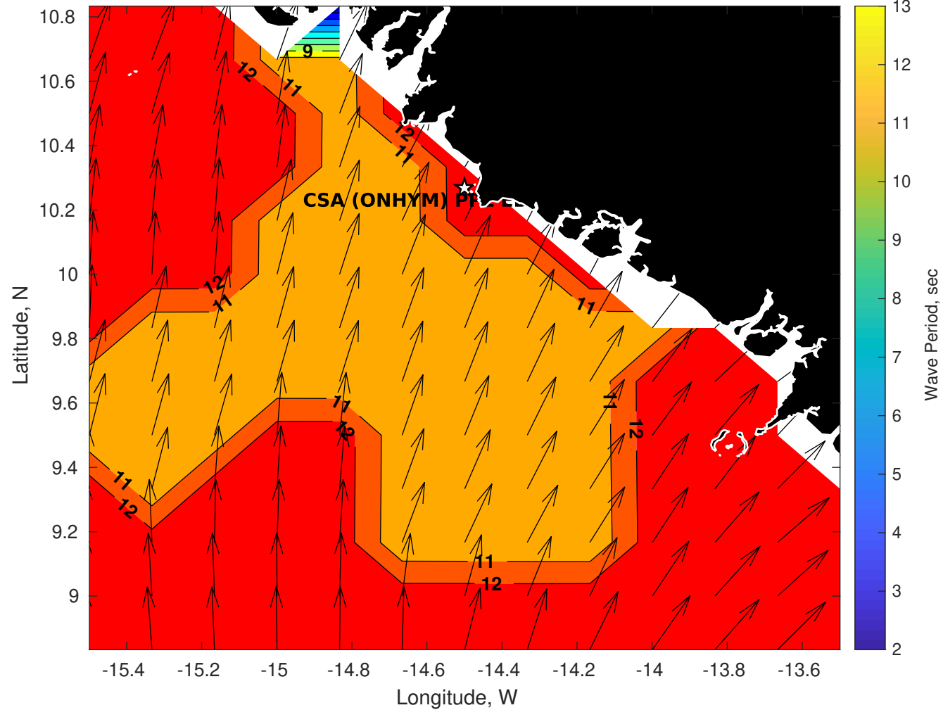
Wave Period (sec) for CSA (ONHYM) PPL EBS - Guinea at 17-Apr-2025 09:00:00
