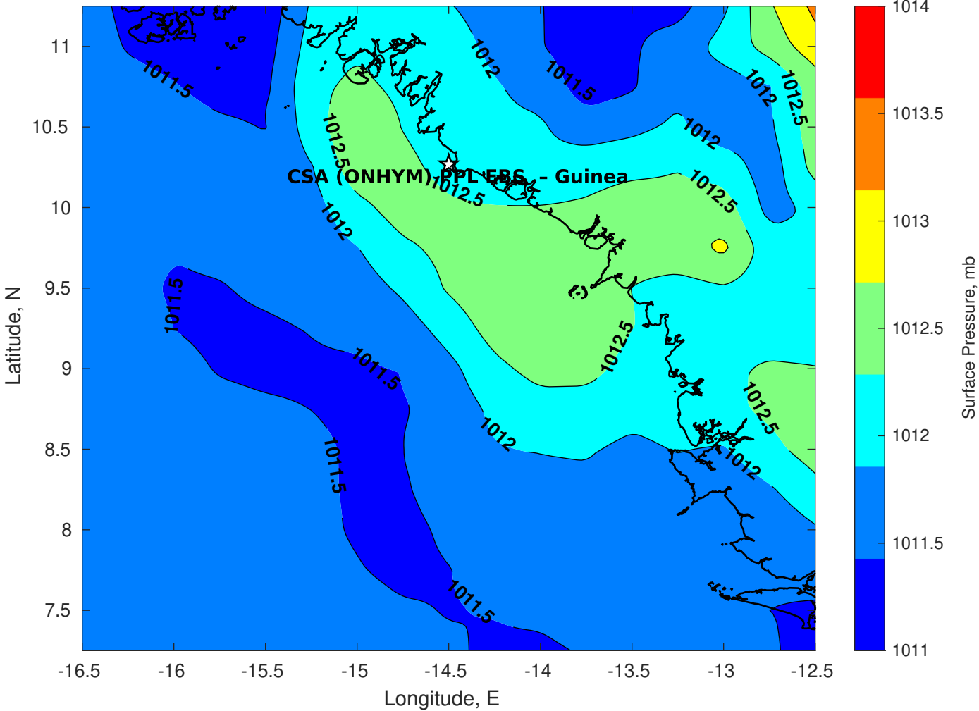
Surface Pressure (mb) for CSA (ONHYM) PPL EBS - Guinea at 19-Apr-2025 00:00:00
