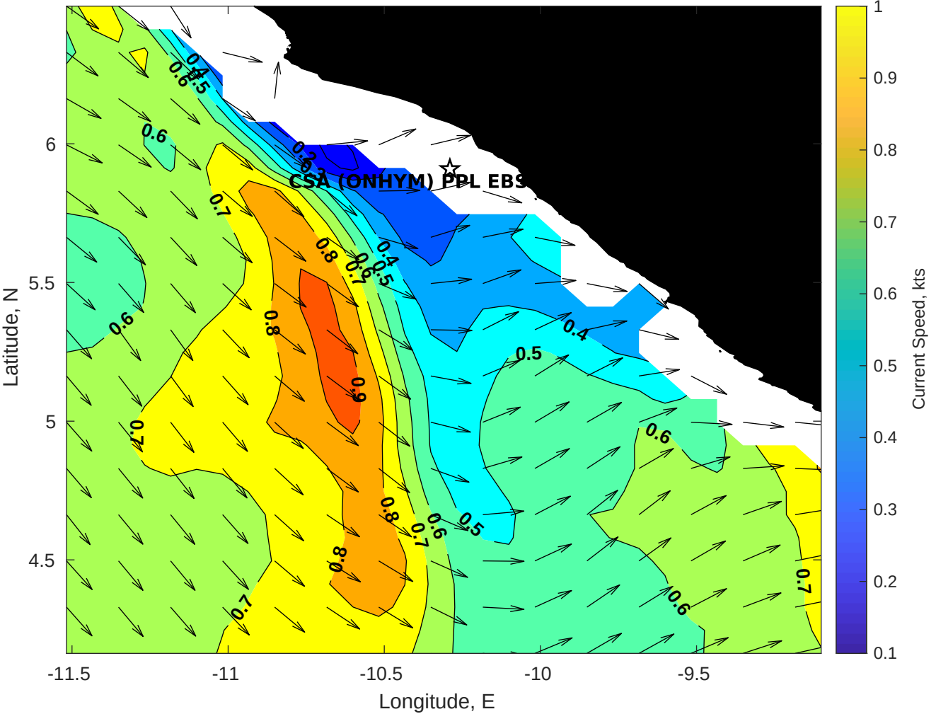
Surface Currents for CSA (ONHYM) PPL EBS - Liberia at 16-Apr-2025 00:00:00
