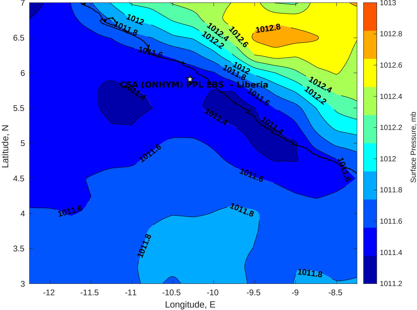
Surface Pressure (mb) for CSA (ONHYM) PPL EBS - Liberia at 17-Apr-2025 00:00:00
