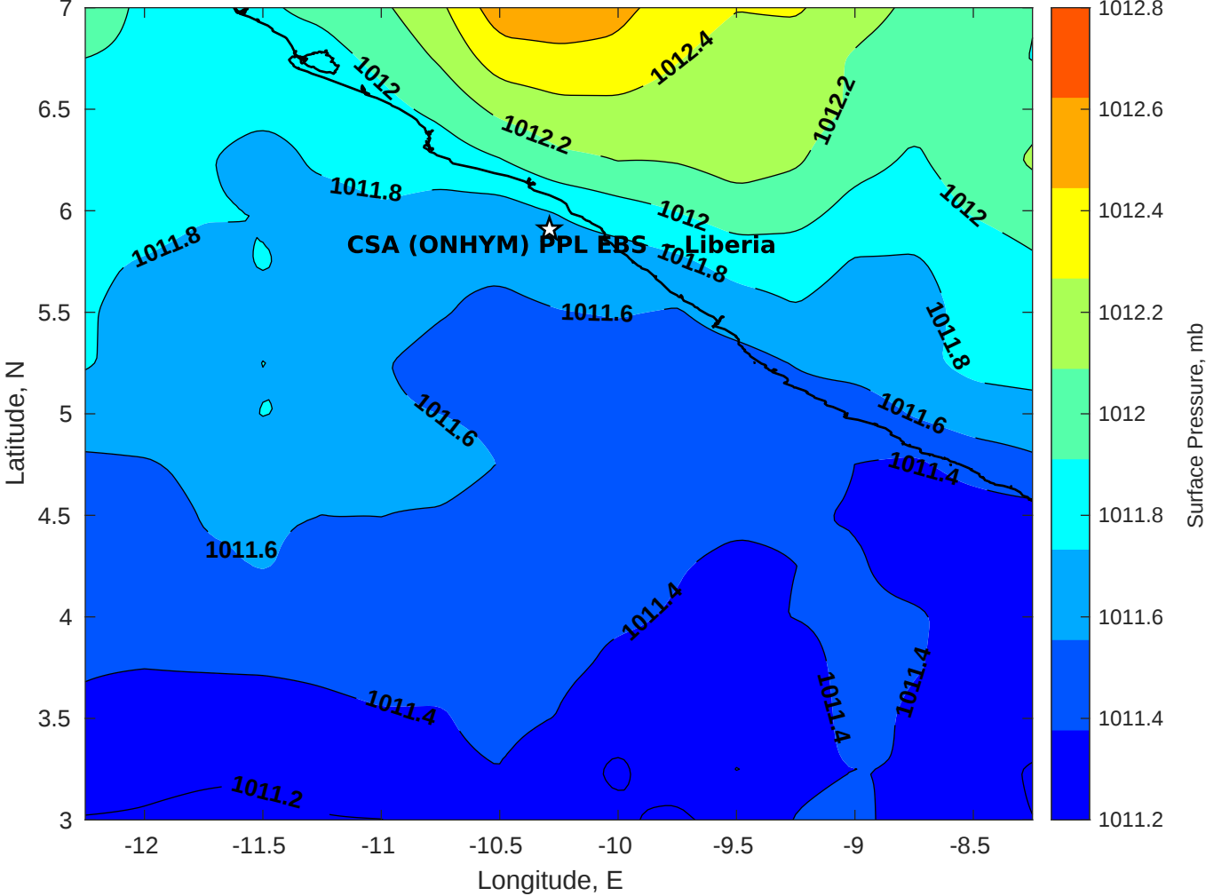
Surface Pressure (mb) for CSA (ONHYM) PPL EBS - Liberia at 18-Apr-2025 00:00:00
