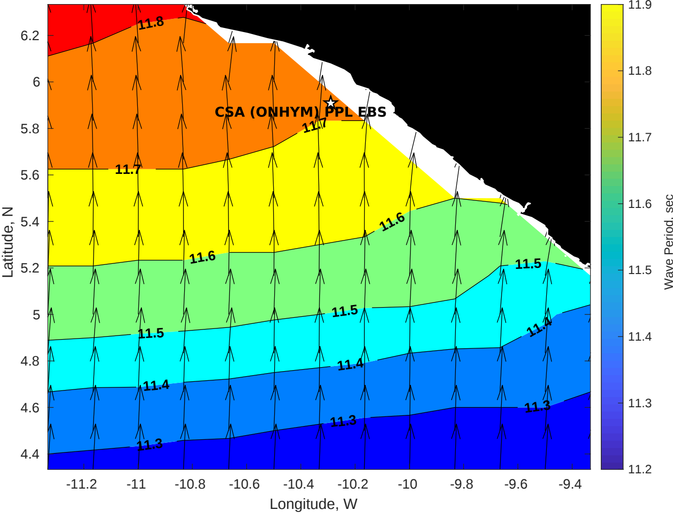
Wave Period (sec) for CSA (ONHYM) PPL EBS - Liberia at 17-Apr-2025 09:00:00
