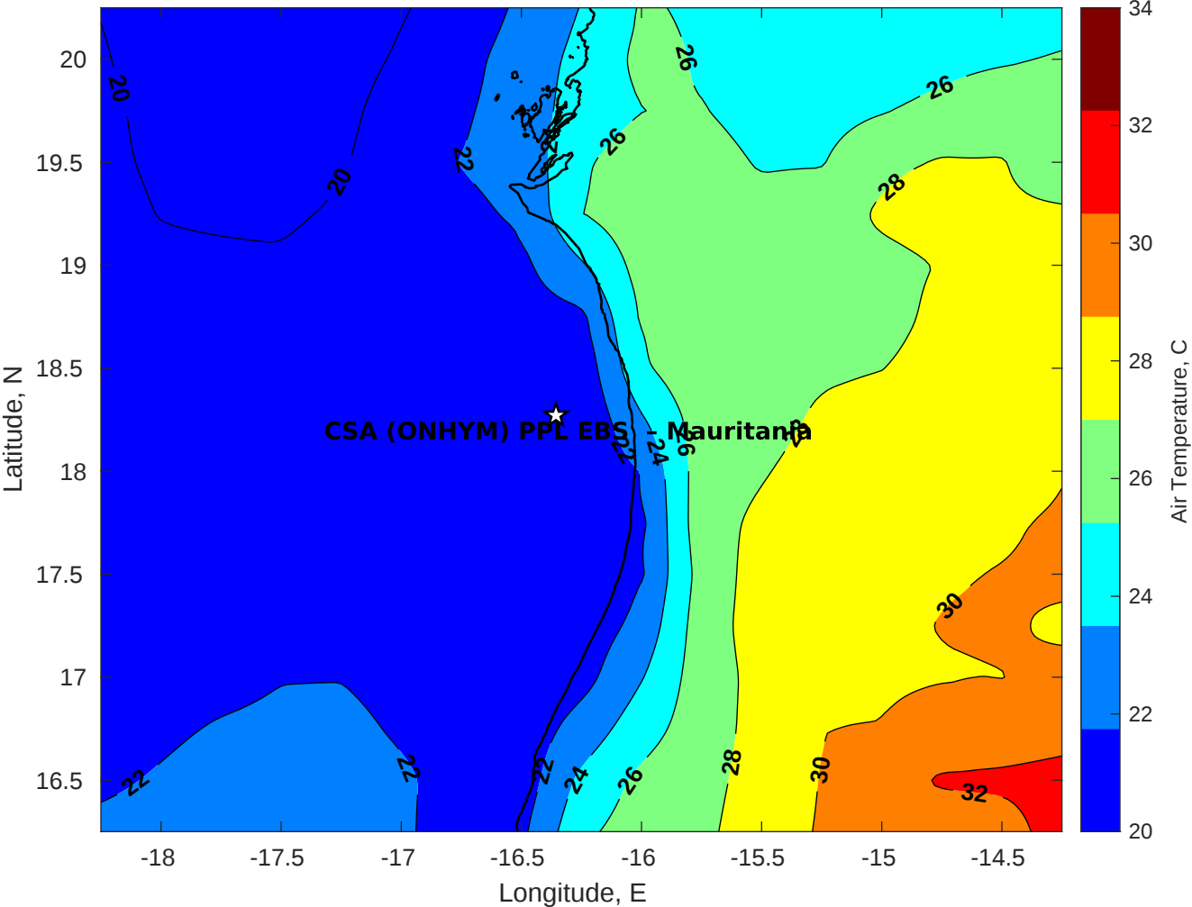
Air Temperature (C) for CSA (ONHYM) PPL EBS - Mauritania at 17-Apr-2025
