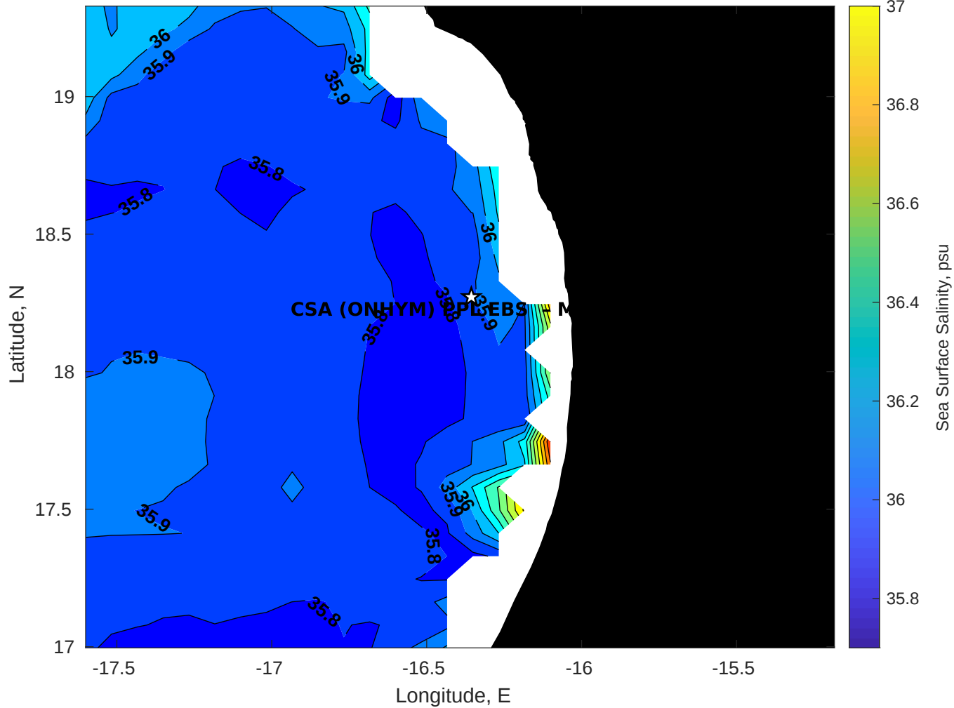
Surface Salinity for CSA (ONHYM) PPL EBS - Mauritania at 16-Apr-2025 00:00:00
