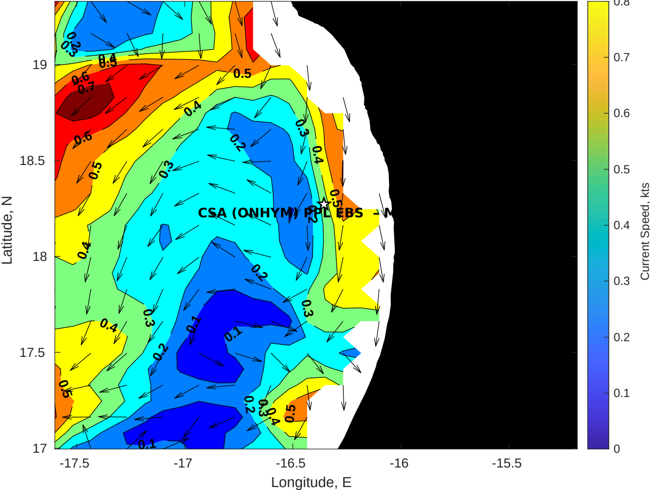
Surface Currents for CSA (ONHYM) PPL EBS - Mauritania at 16-Apr-2025 00:00:00
