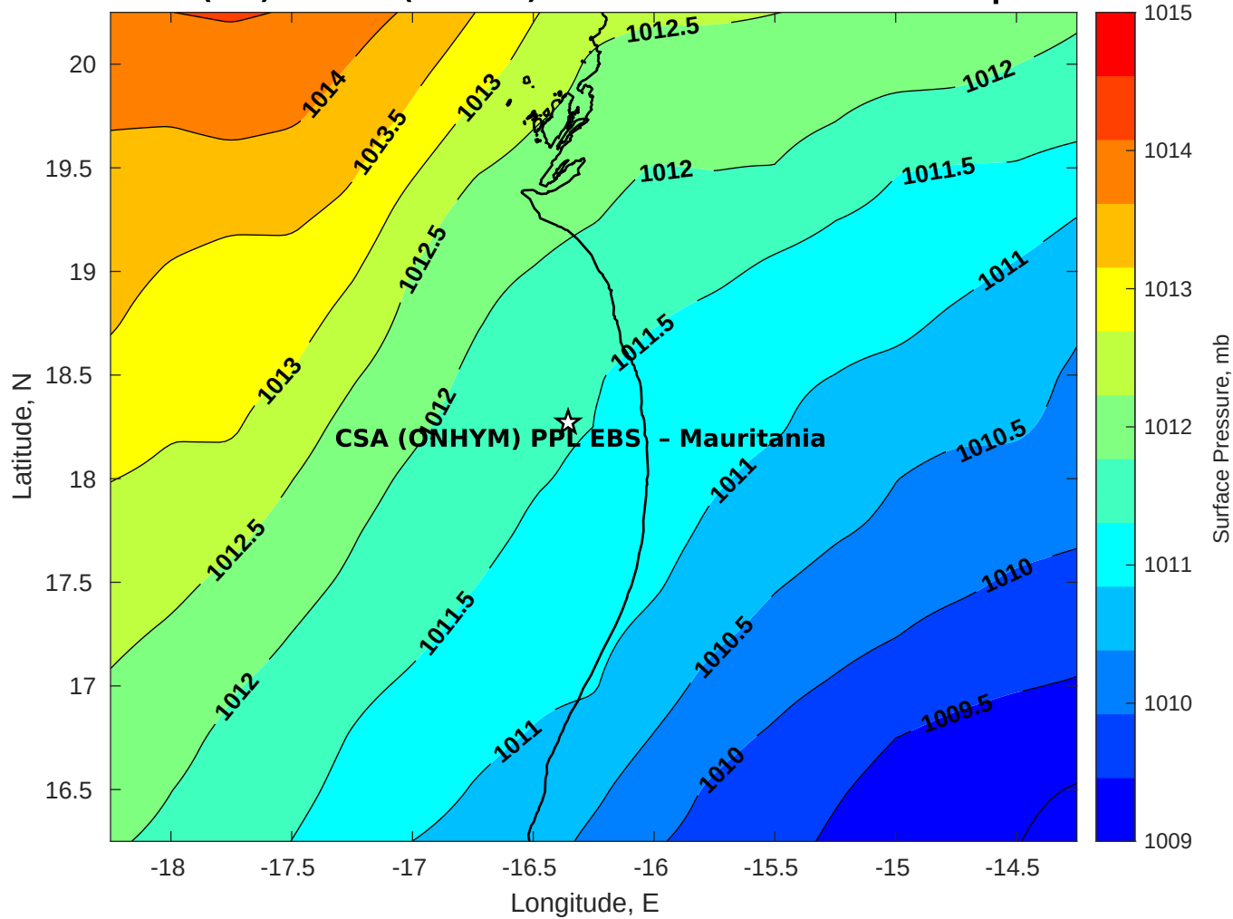
Surface Pressure (mb) for CSA (ONHYM) PPL EBS - Mauritania at 17-Apr-2025 00:00:00
