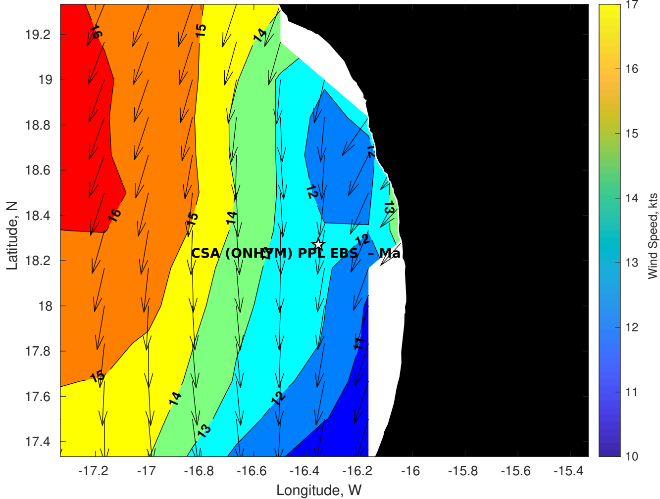
Winds (kts) for CSA (ONHYM) PPL EBS - Mauritania at 17-Apr-2025 09:00:00
