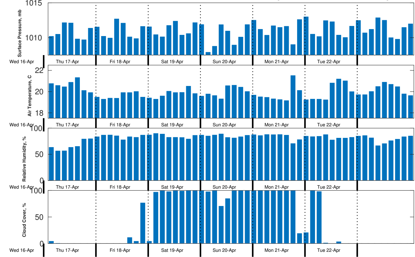
Met Forecast for CSA (ONHYM) PPL EBS - Mauritania from 17-Apr-2025 00:00:00 to 24-Apr-2025 00:00:00
