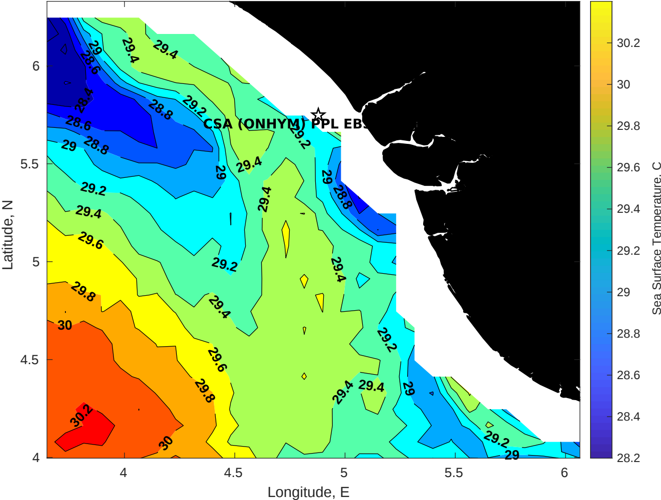
SST for CSA (ONHYM) PPL EBS - Nigeria at 16-Apr-2025 00:00:00
