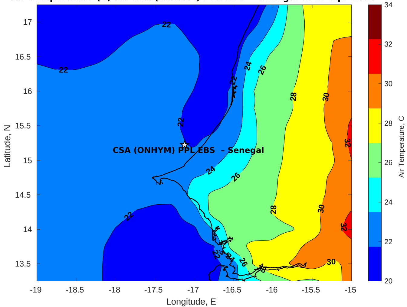
Air Temperature (C) for CSA (ONHYM) PPL EBS - Senegal at 17-Apr-2025
