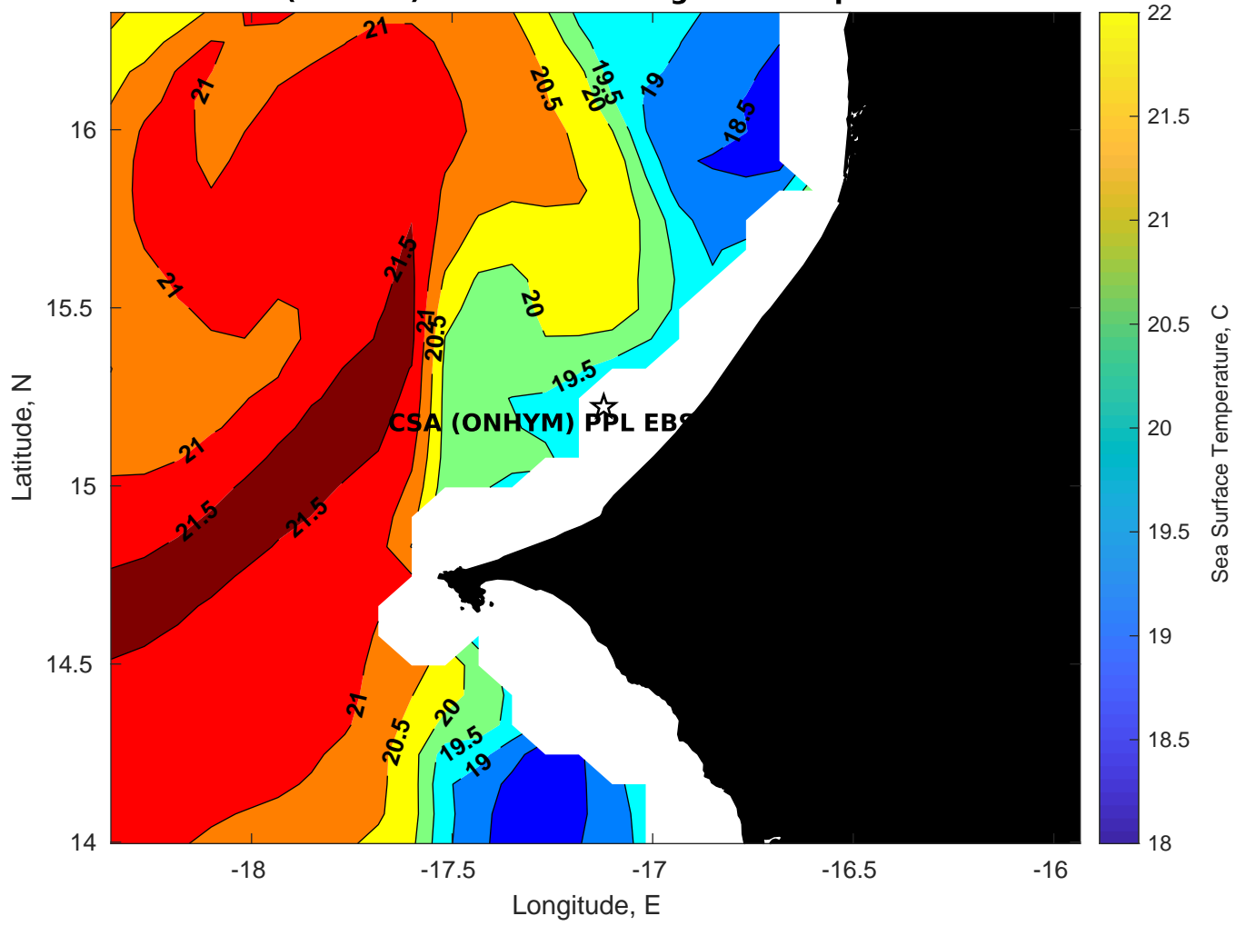
SST for CSA (ONHYM) PPL EBS - Senegal at 16-Apr-2025 00:00:00
