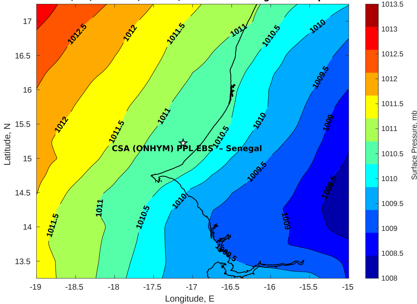
Surface Pressure (mb) for CSA (ONHYM) PPL EBS - Senegal at 17-Apr-2025 00:00:00
