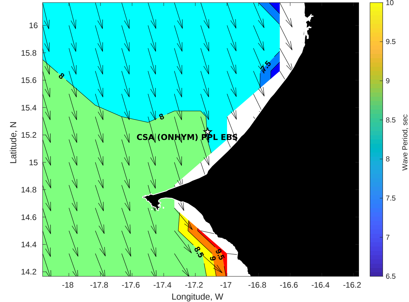
Wave Period (sec) for CSA (ONHYM) PPL EBS - Senegal at 17-Apr-2025 09:00:00
