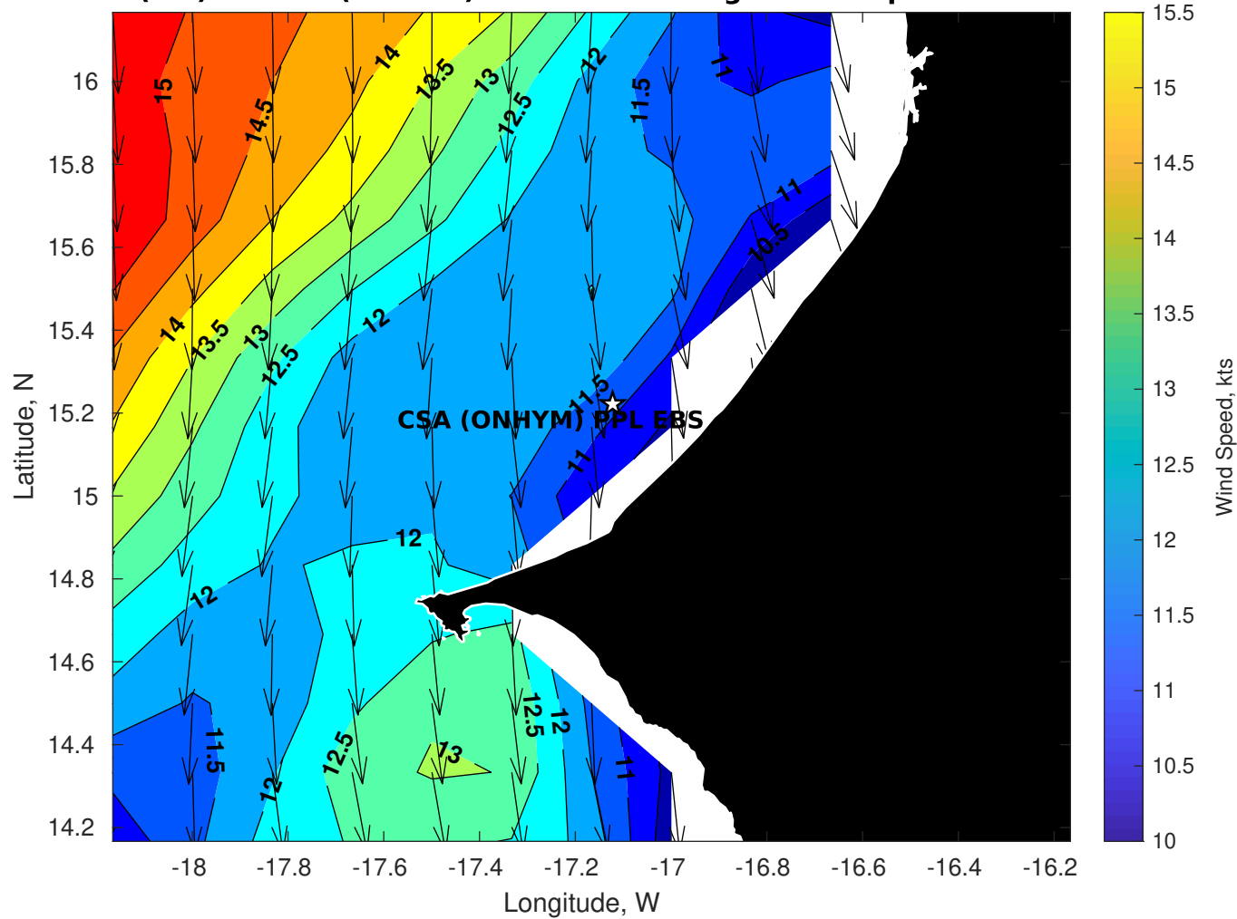
Winds (kts) for CSA (ONHYM) PPL EBS - Senegal at 17-Apr-2025 09:00:00
