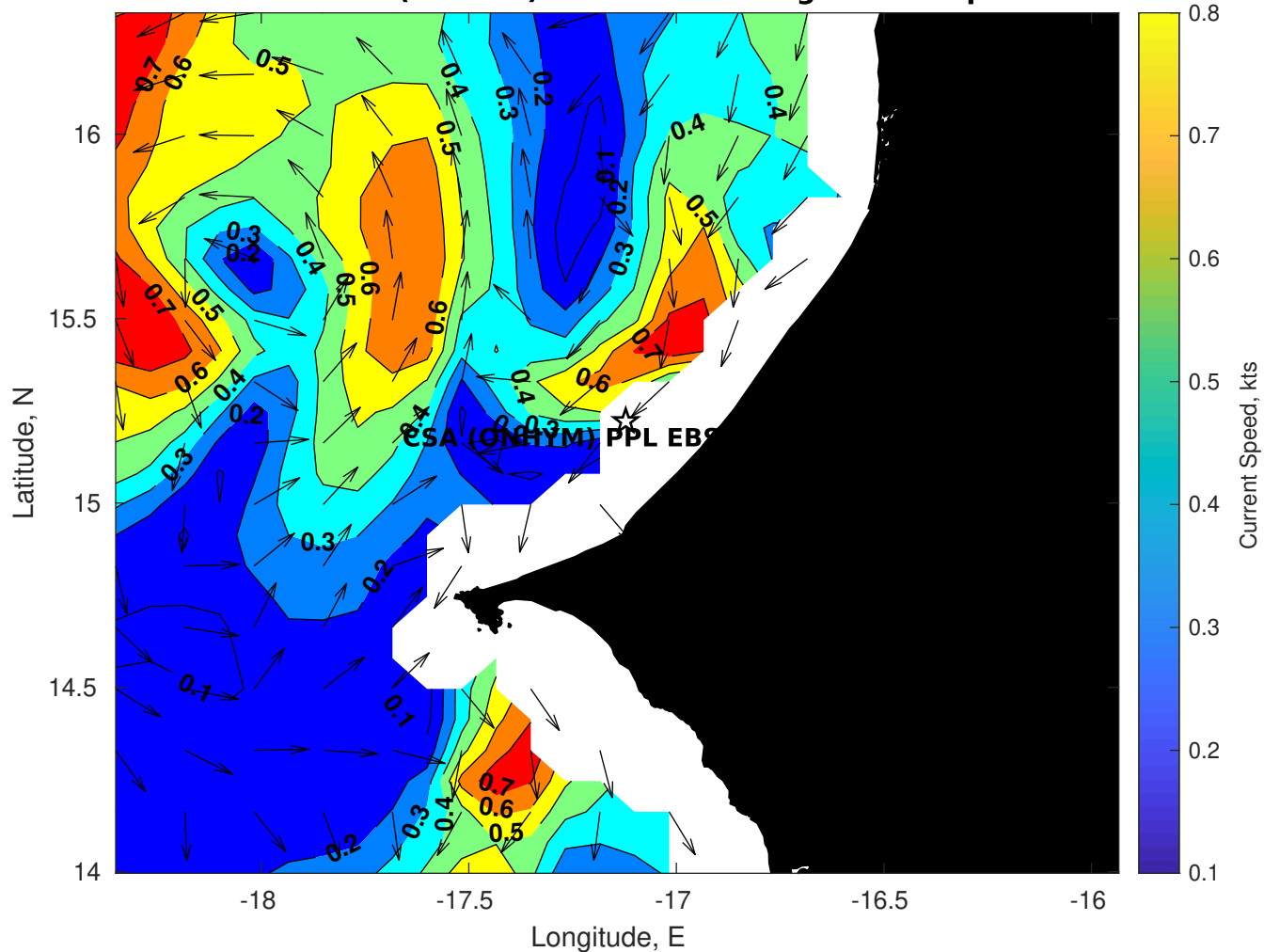
Surface Currents for CSA (ONHYM) PPL EBS - Senegal at 16-Apr-2025 00:00:00
