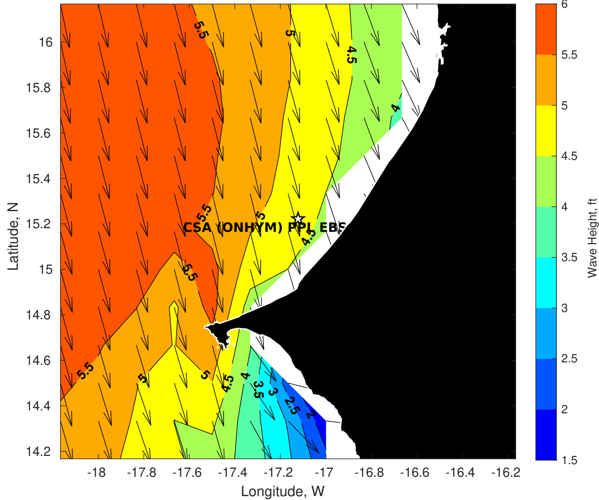
Wave Height (ft) for CSA (ONHYM) PPL EBS - Senegal at 17-Apr-2025 09:00:00
