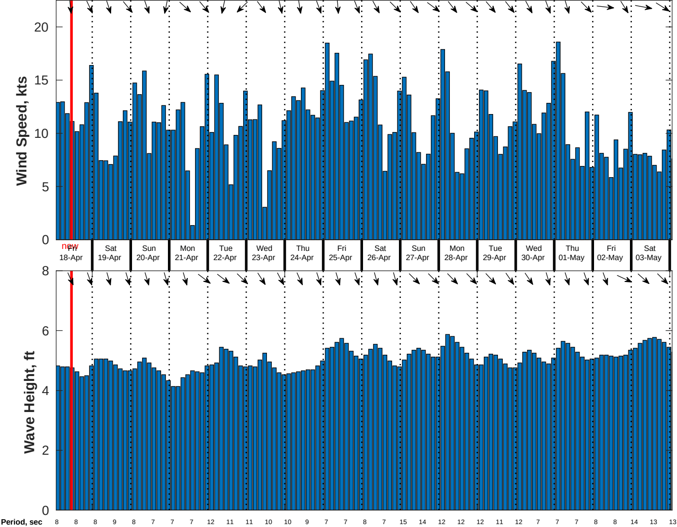
Wind & Wave Forecast for CSA (ONHYM) PPL EBS - Senegal from 17-Apr-2025 01:00:00 to 03-May-2025 01:00:00
