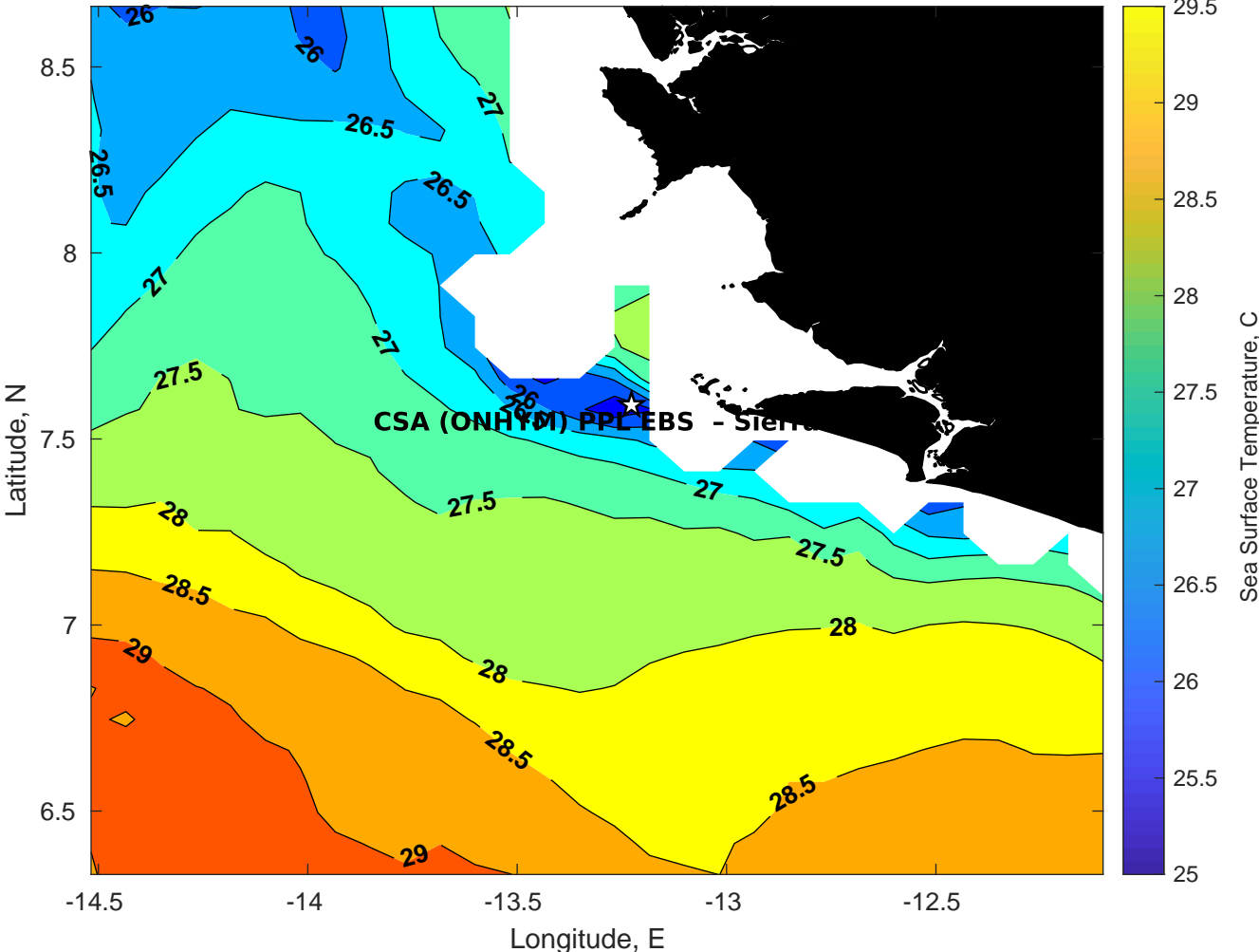
SST for CSA (ONHYM) PPL EBS - Sierra Leone at 16-Apr-2025 00:00:00
