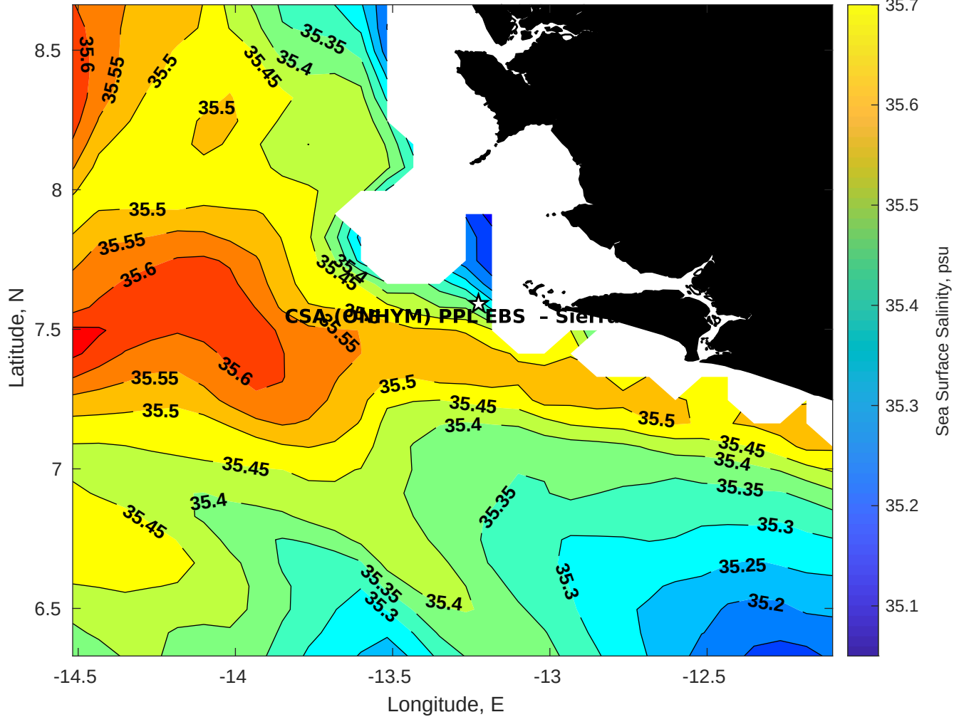
Surface Salinity for CSA (ONHYM) PPL EBS - Sierra Leone at 16-Apr-2025 00:00:00
