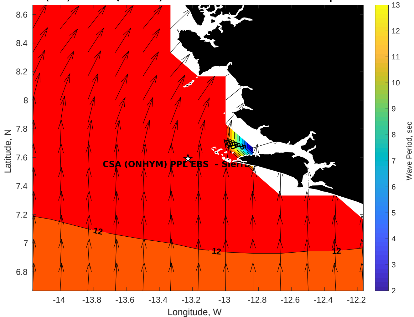
Wave Period (sec) for CSA (ONHYM) PPL EBS - Sierra Leone at 17-Apr-2025 09:00:00
