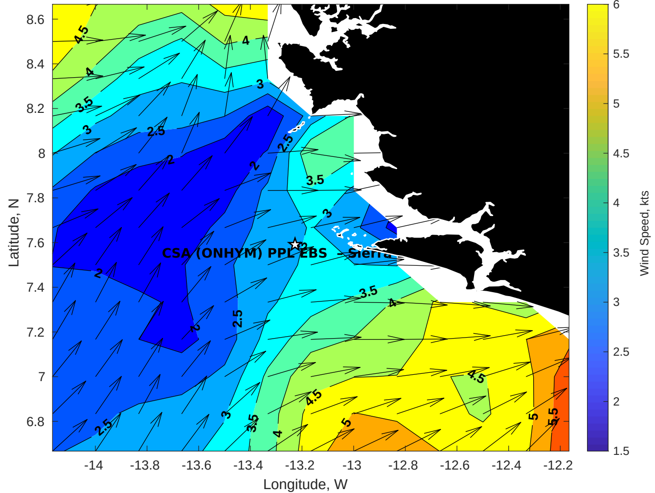
Winds (kts) for CSA (ONHYM) PPL EBS - Sierra Leone at 17-Apr-2025 09:00:00
