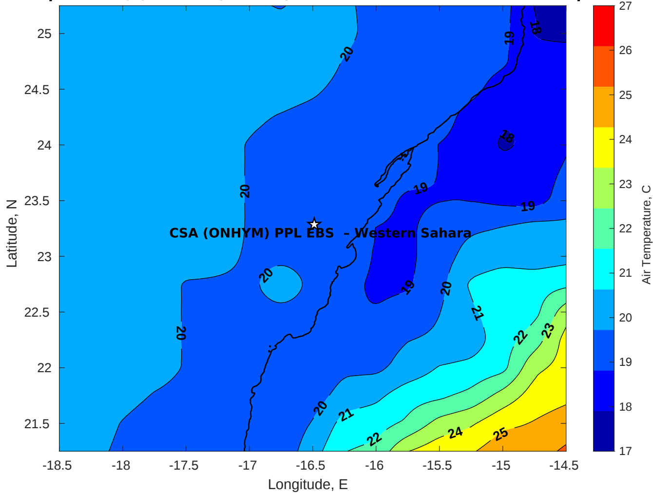
Air Temperature (C) for CSA (ONHYM) PPL EBS - Western Sahara at 17-Apr-2025
