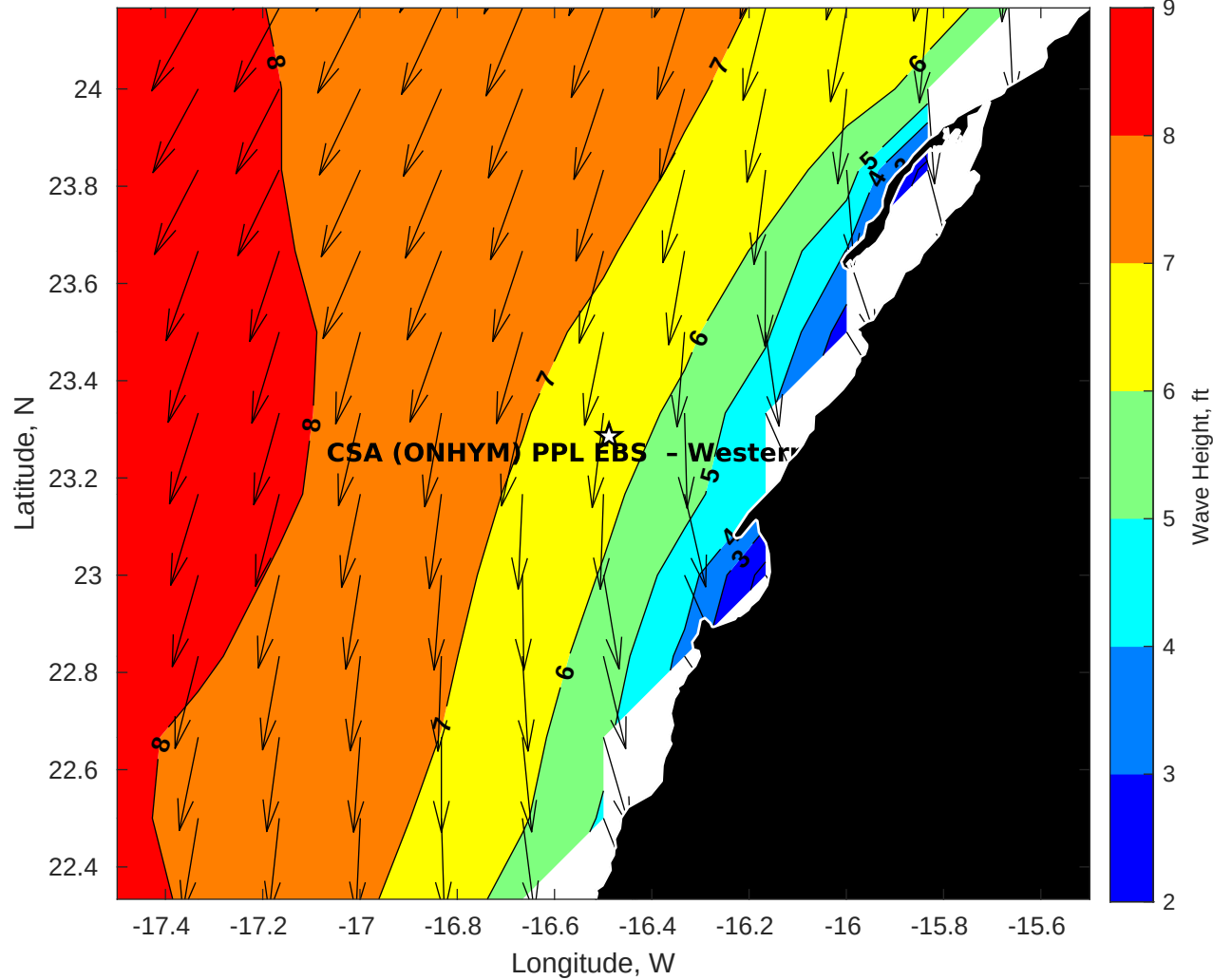
Wave Height (ft) for CSA (ONHYM) PPL EBS - Western Sahara at 17-Apr-2025 09:00:00
