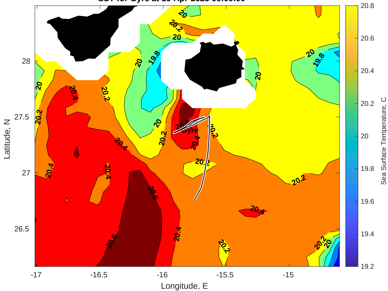
SST for Gyre at 16-Apr-2025 00:00:00
