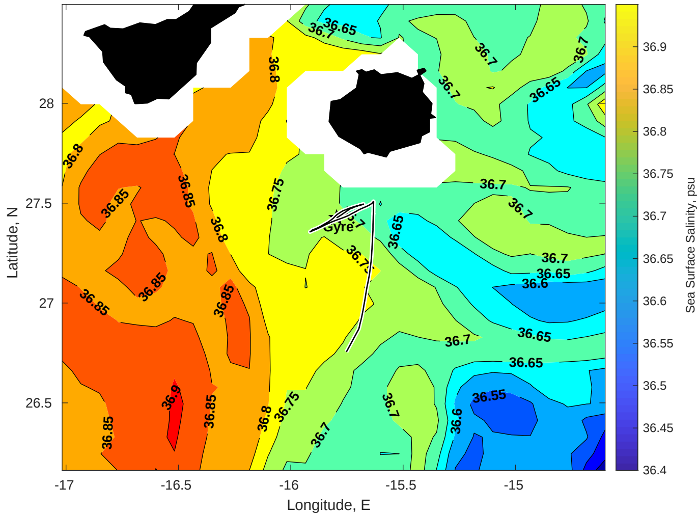
Surface Salinity for Gyre at 16-Apr-2025 00:00:00
