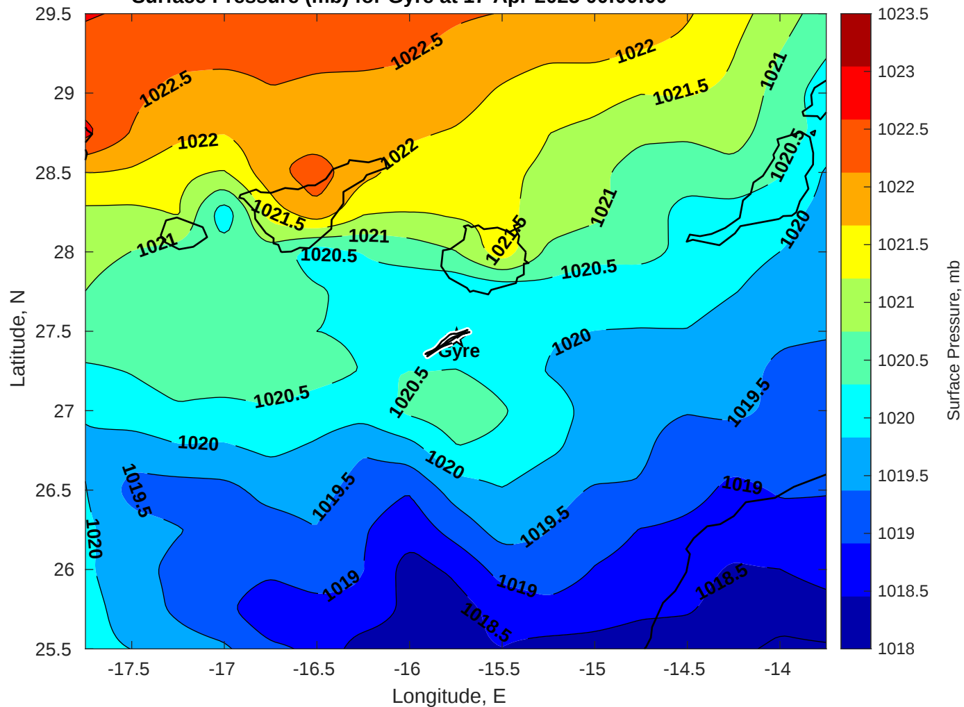
Surface Pressure (mb) for Gyre at 17-Apr-2025 00:00:00
